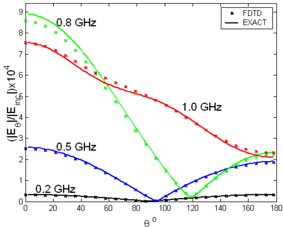
Fig. 7 Scattering from a chiral sphere, \varepsilon_r = 4 , \chi = 0.5 .
