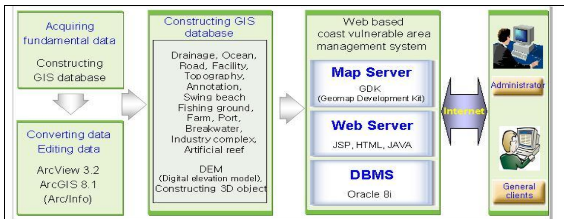
Fig. 3. The concept diagram of system development
