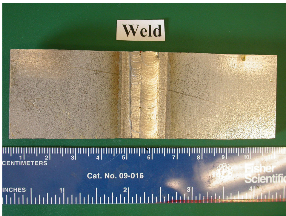
Figure 2. 304L/Monel weld after 50 days exposure in aerated artificial seawater.
