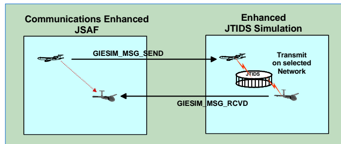
Figure 4-4. Message Transmission Request and Response
