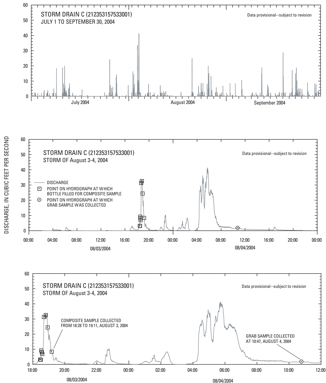
Figure 3. Discharge at Storm drain C station (212353157533001) for July 1 to September 30, 2004; detail of the 2-day period of August 3-4, 2004; and detail of the 18-hour period from 18:00 August 3, 2004 to 12:00 August 4, 2004, Oahu, Hawaii.
