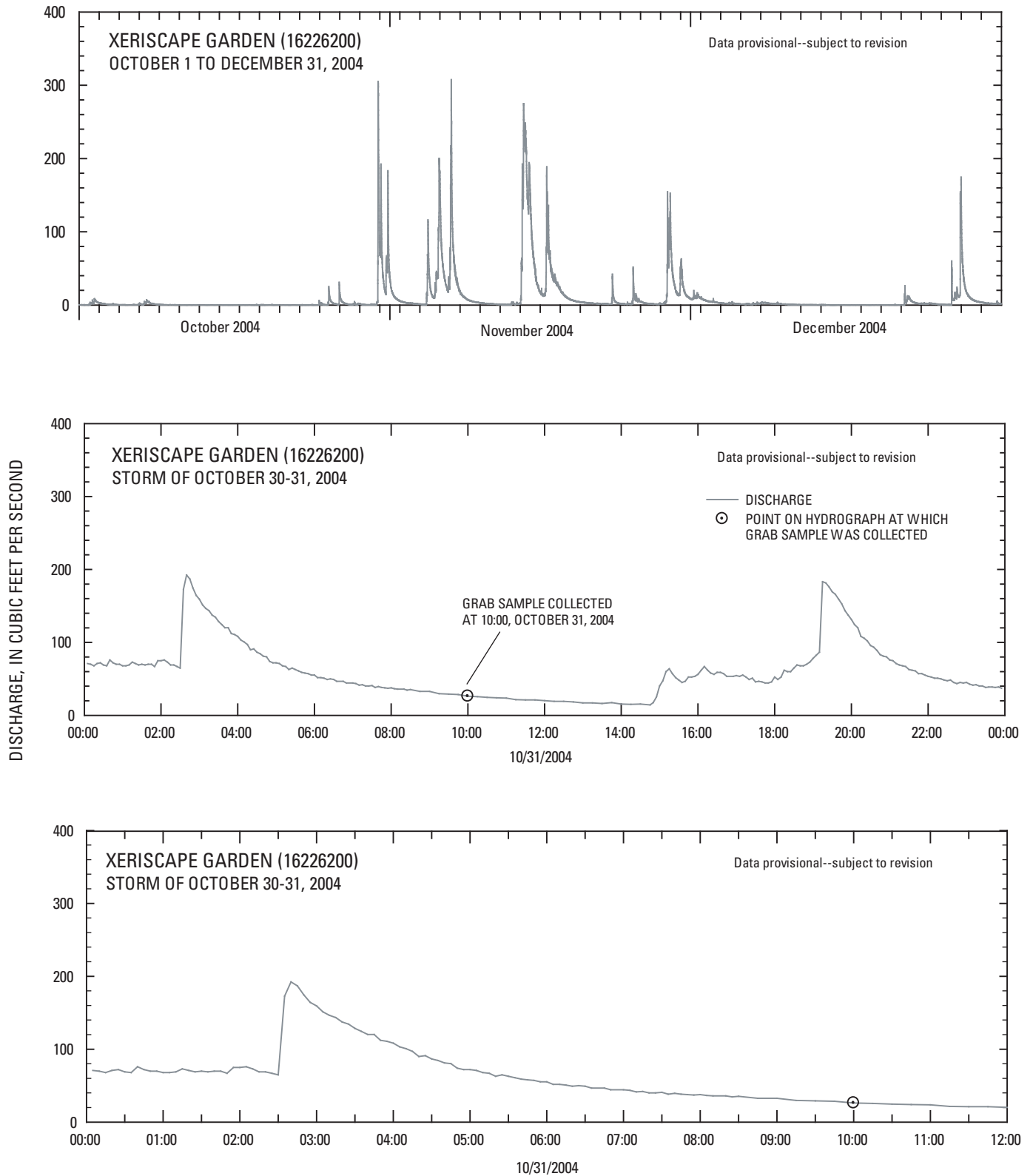
Figure 6. Stream discharge at Xeriscape garden station (16226200) for October 1 to December 31, 2004; detail of the 1-day period of October 31, 2004; and detail of the 12-hour period from 00:00 to 12:00 October 31, 2004, Oahu, Hawaii.
