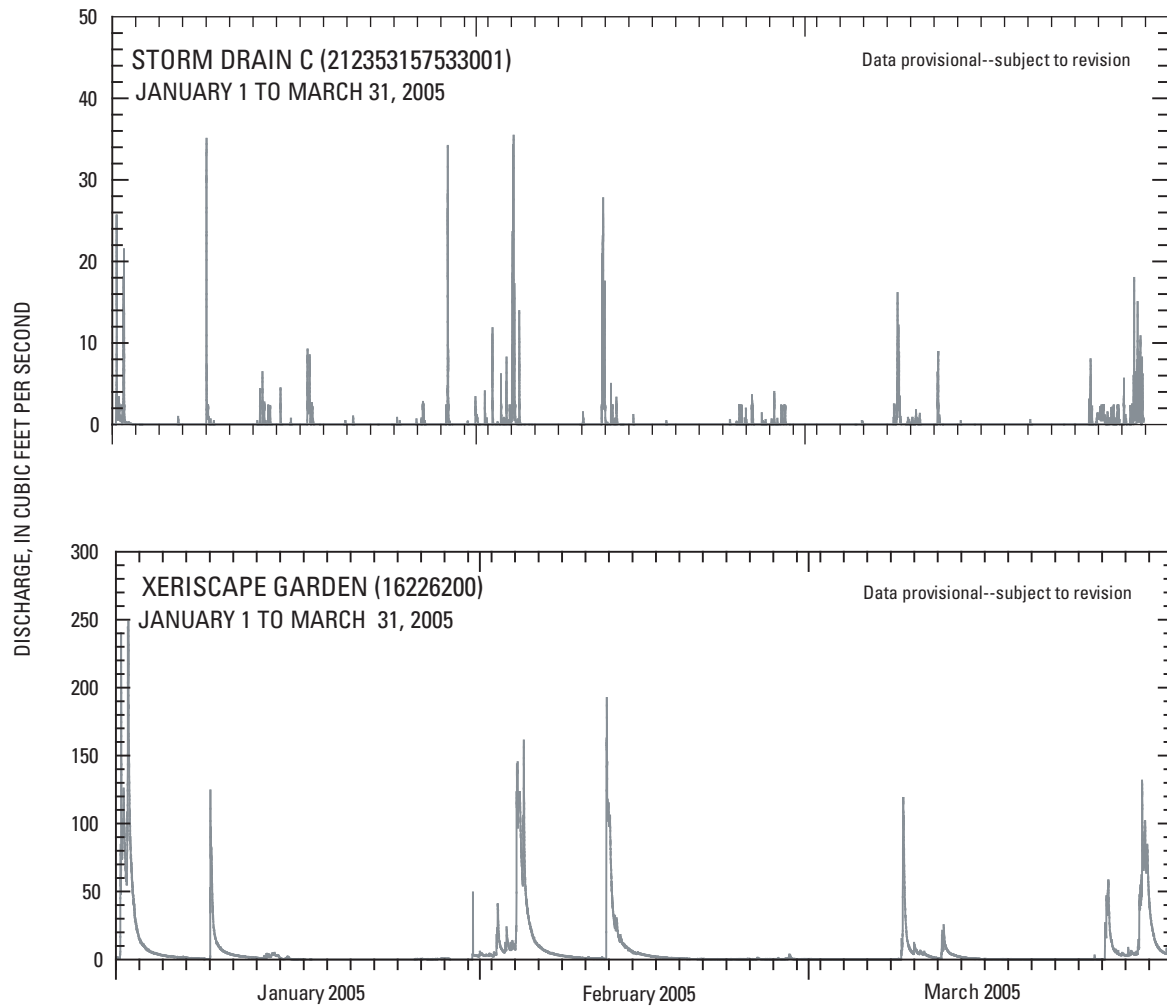
Figure 9. Discharge at Storm drain C (212353157533001) and Xeriscape garden (16226200) stations for January 1 to March 31, 2005, Oahu, Hawaii.
