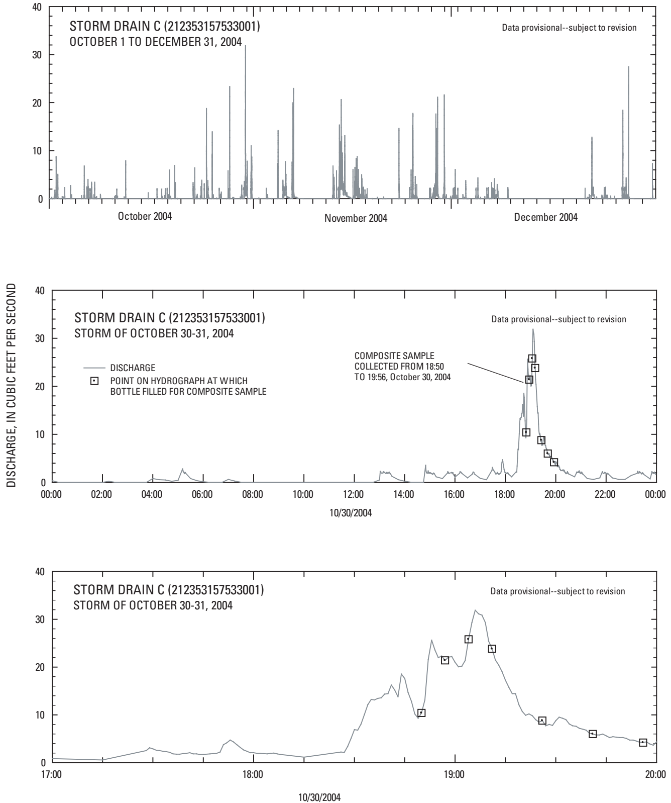
Figure 5. Discharge at Storm drain C station (212353157533001) for October 1 to December 31, 2004; detail of the 1-day period of October 30, 2004; and detail of the 3-hour period from 17:00 to 20:00 October 30, 2004, Oahu, Hawaii.
