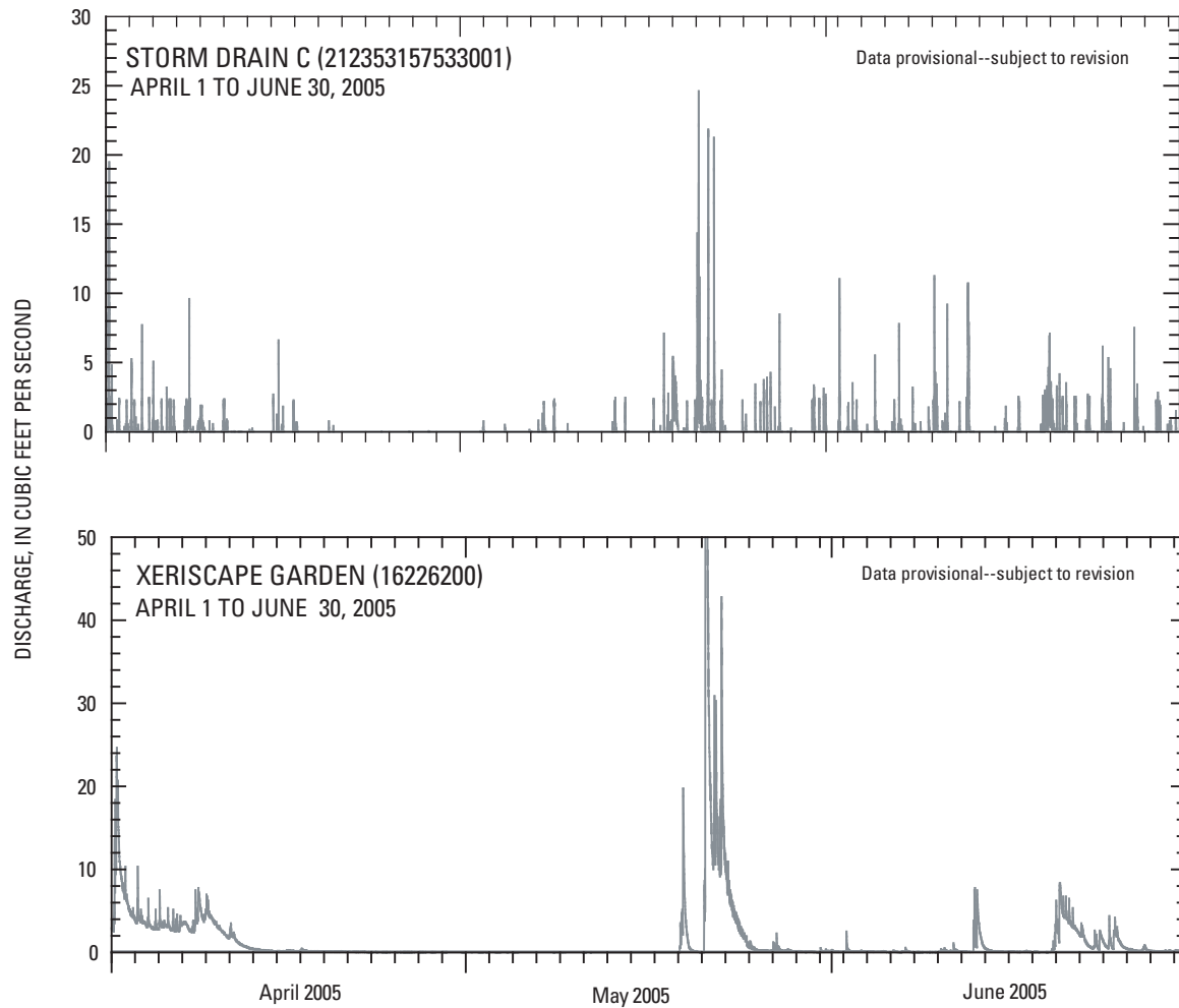
Figure 10. Stream discharge at Storm drain C (212353157533001) and Xeriscape garden (16226200) stations for April 1 to June 30, 2005, Oahu, Hawaii.
