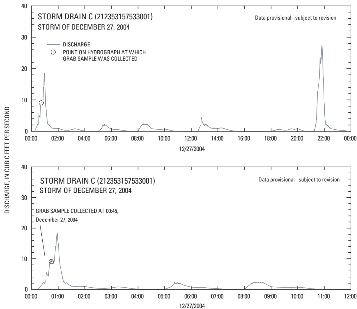
Figure 7. Discharge at Storm drain C station (212353157533001) for the 1-day period of December 27, 2004; and detail of the 12-hour period from 00:00 to 12:00 December 27, 2004, Oahu, Hawaii.
