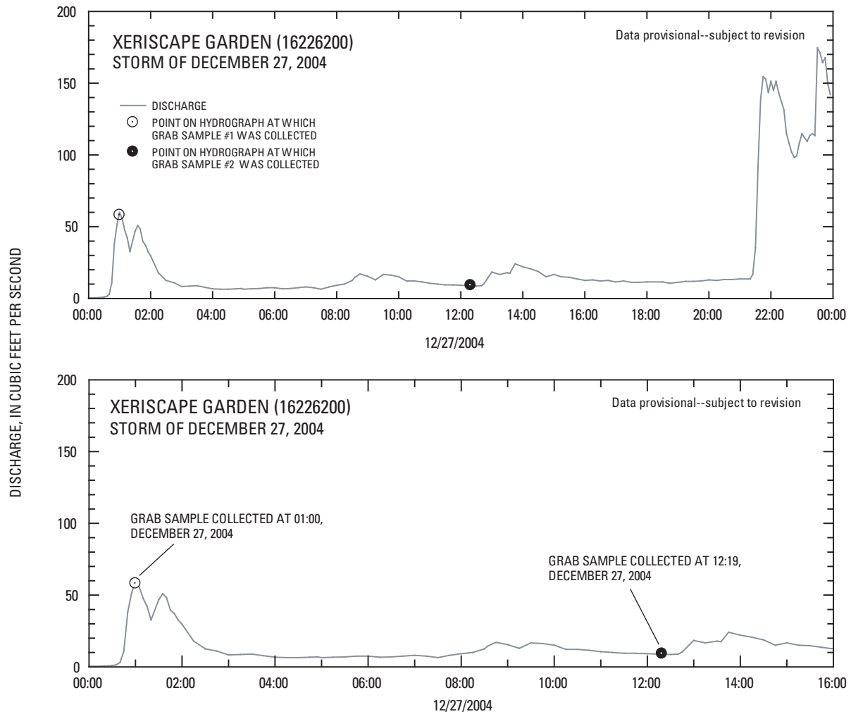
Figure 8. Stream discharge at Xeriscape garden station (16226200) for 1-day period of December 27, 2004; and detail of the 16-hour period from 00:00 to 16:00 December 27, 2004, Oahu, Hawaii.
