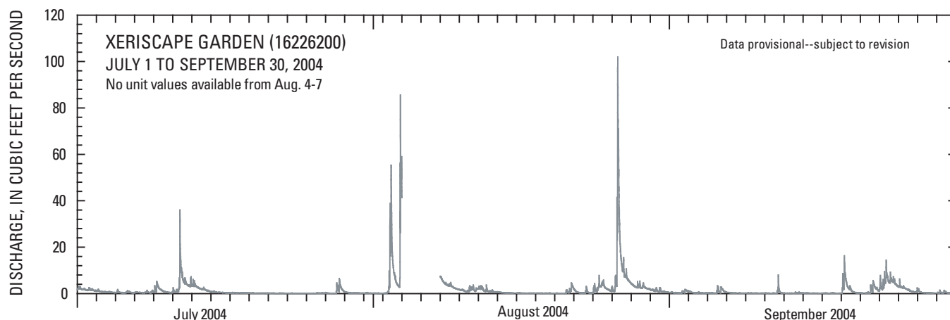
Figure 4. Stream discharge at Xeriscape garden station (16226200) for July 1 to September 30, 2004, Oahu, Hawaii.
