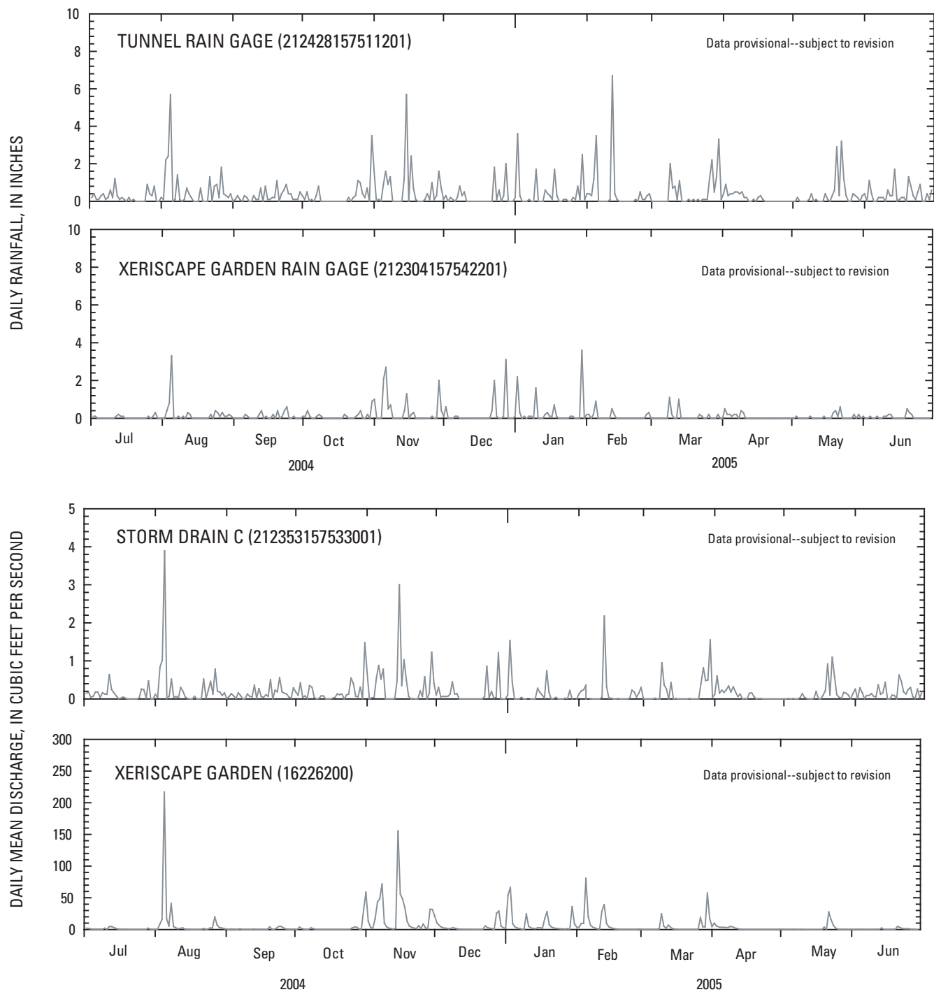
Figure 2. Rainfall and discharge for stations within the Halawa Stream drainage basin, Oahu, Hawaii, for July 1, 2004 to June 30, 2005.
