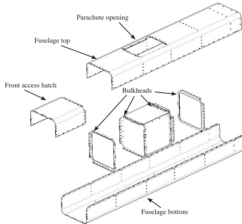
Fig. 15 — Fuselage parts
