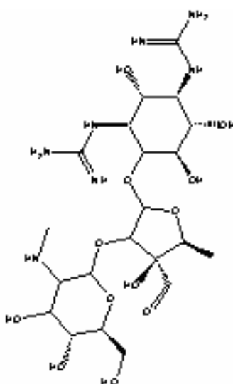
Figure 13. Streptomycin molecule. (27).
