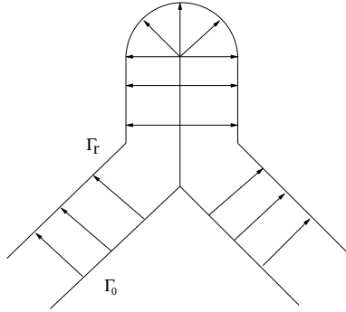
Figure 3: Characteristics in pseudo-reinitialization.
