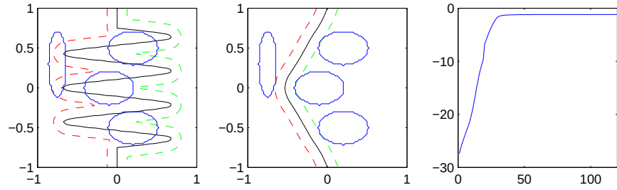
Figure 10: Initial, steady state and energy vs. timesteps plots for object avoidance. Solution converges to global minimum.
