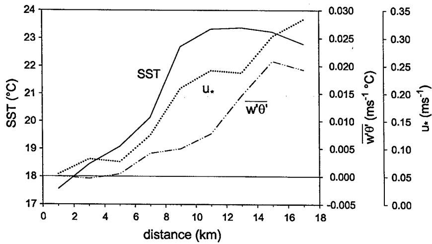
Figure 4. The spatial variation of the SST, friction velocity and heat flux at 33 m near the main SST front on 20 November. The values are composited over the 5 passes. The compositing causes some spatial spreading because the individual records are not perfectly aligned with respect to the SST front. The flow is from left to right.
