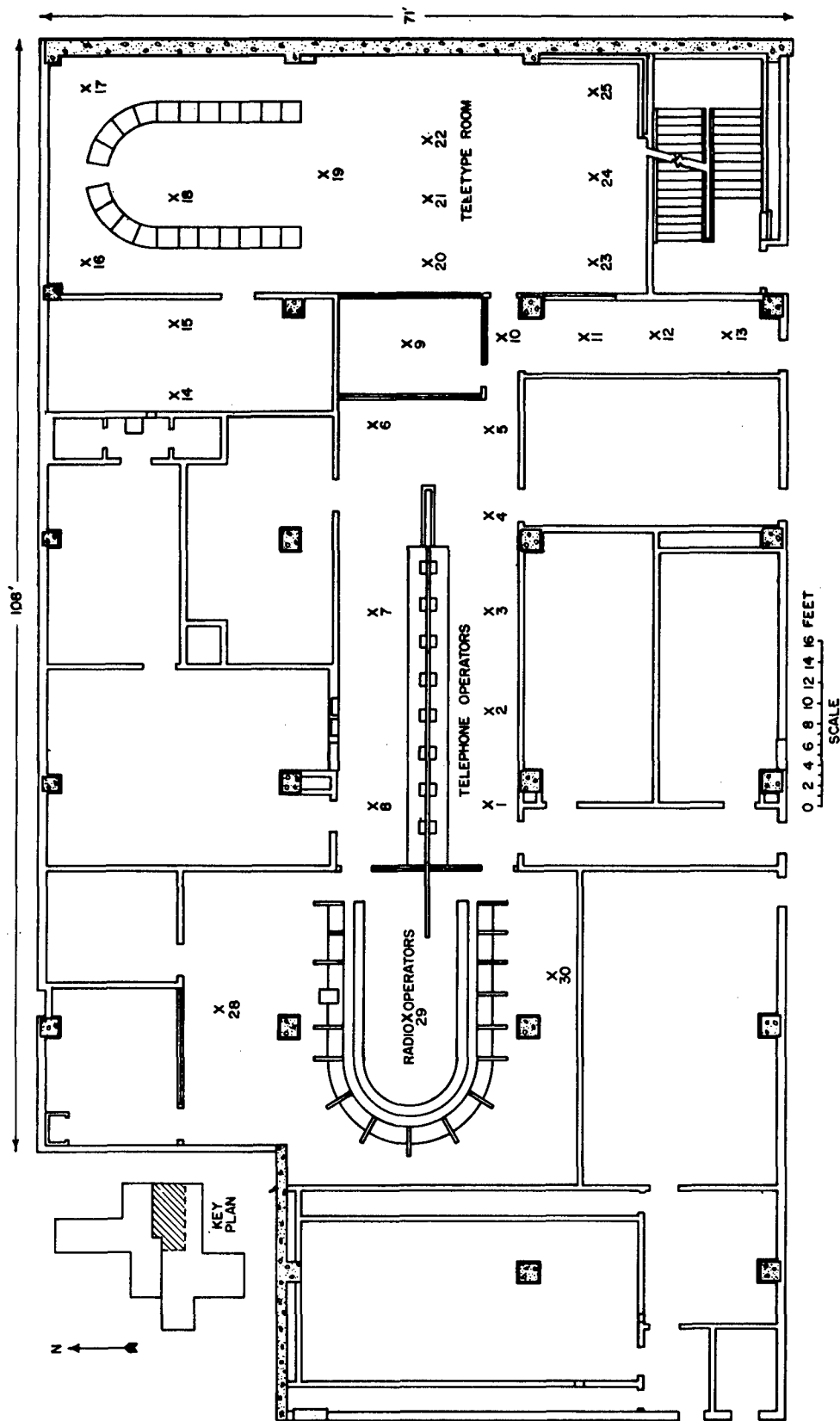
Fig. 3.5—Floor plan of communications section of Los Angeles Police Department building showing detector positions.
