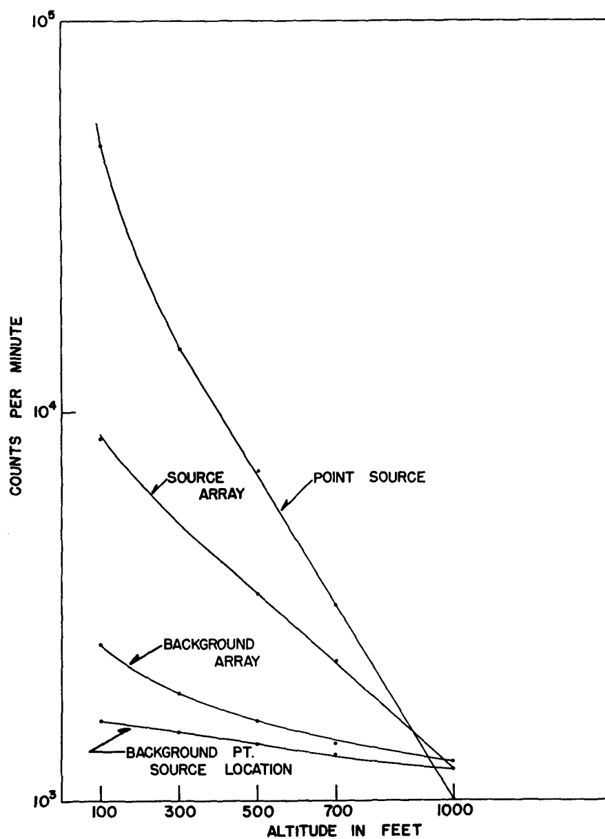
Fig. 6.2—Aerial radiometric measurements of \text{Co}^{60} sources made with bio-plastic detector.
