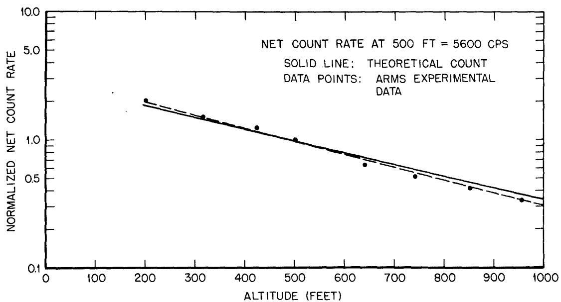
Fig. 3.2— \text{Cs}^{137} -array normalized count rate vs. altitude.
