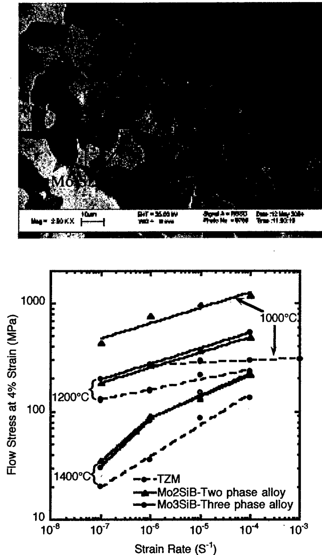
Figure 10: a) Back-scattered electron image of the three-phase Mo-8.6Si-8.7B alloy confirming the presence of the matrix solid solution phase and two types of precipitate phases that were verified by x-ray diffraction and compositional analyses to be the T2 phase and the \text{Mo}_3\text{Si} phase as labeled. In b) a comprehensive comparison is made of the variation of compressive flow stress at 4% strain for T-ZM, Mo-6.1Si-7.9B and Mo-8.6Si-8.7B with nominal strain rate in the strain rate regime 10^{-4} \text{ s}^{-1} to 10^{-7} \text{ s}^{-1} at test temperatures of 1000°C, 1200°C and 1400°C.
