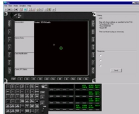
Figure 3. Simulation interface
