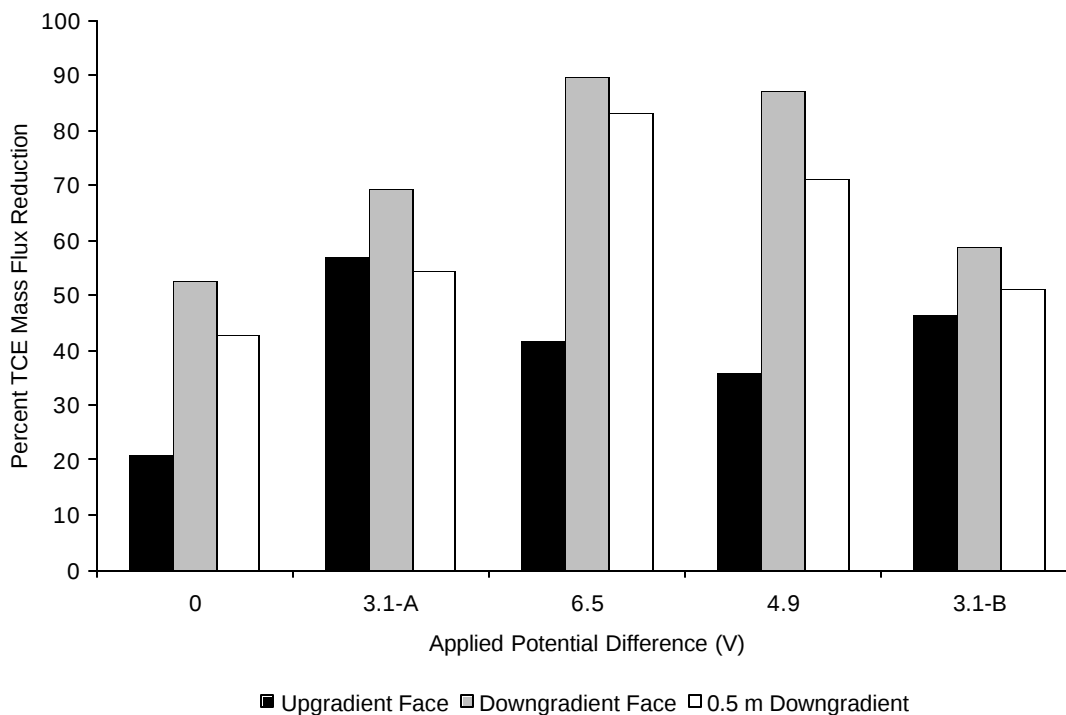
Figure 42. Barrier-wide percent TCE mass flux reduction at each E_{appl} tested during the demonstration. The settings appear in chronological order from left to right on the x-axis, such that 3.1 V-A took place before 3.1 V-B.
