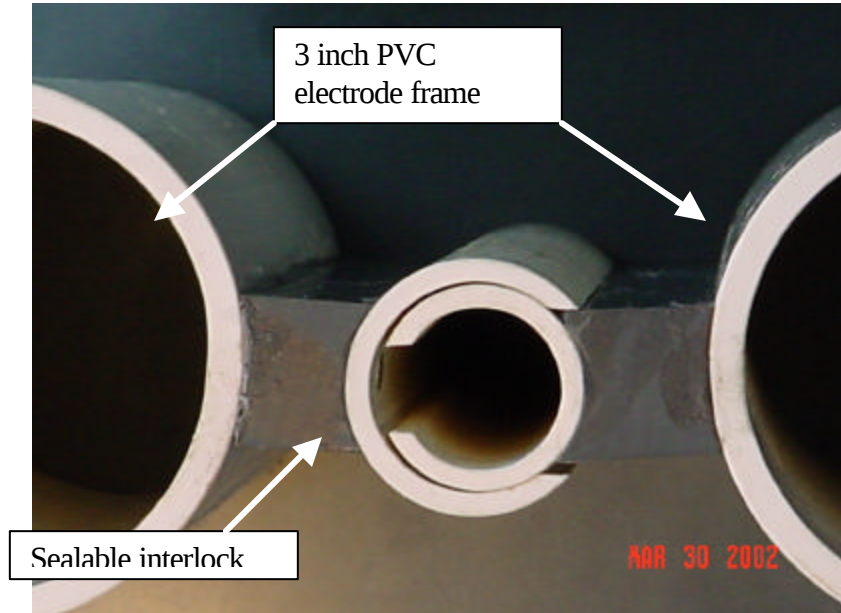
Figure 11 –Panel interlock
