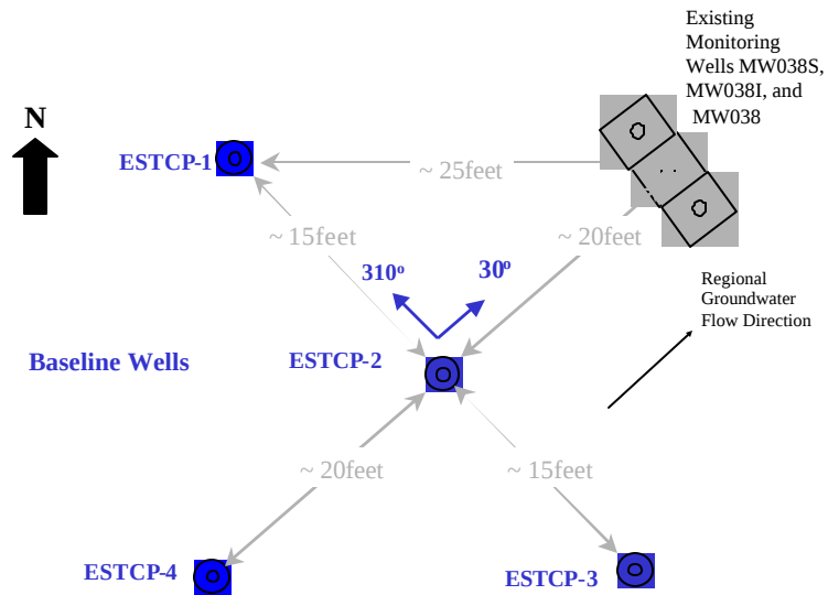
Figure 4. Layout of existing and temporary wells at the selected demonstration location
