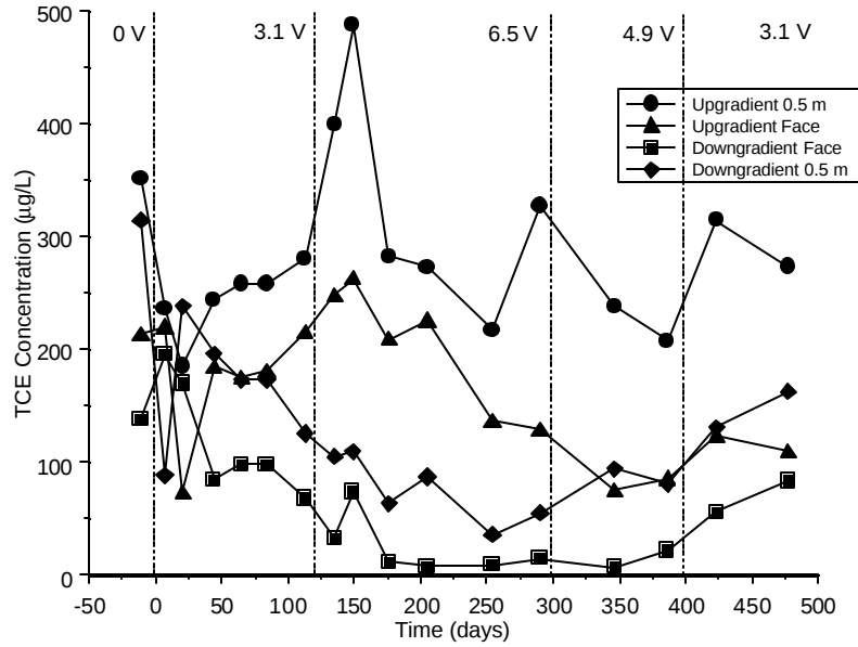
Figure 45. Average TCE concentrations along the transect parallel to groundwater flow at the e-barrier midpoint. Values are arranged from 0.5 m upgradient of the barrier (circles), upgradient face of the barrier (triangles), downgradient face of the barrier (boxes), and 0.5 m downgradient of the barrier (diamonds). Power was applied to the e-barrier at day 0.
