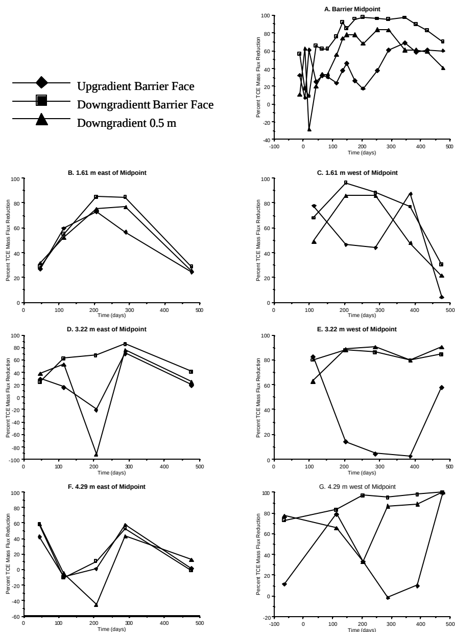
Figure 39. Percent TCE mass flux reduction at the upgradient e^- barrier face (diamonds), downgradient e^- barrier face (boxes), and 0.5 m downgradient (triangles) locations. Each location is from a perpendicular plane the stated distance from the e^- barrier midpoint. Power was applied to the e^- barrier at day 0.
