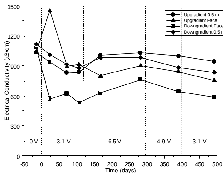
Figure 49. Electrical conductivity measured along the transect parallel to flow at the e^- barrier midpoint. Measurements are averaged from readings taken 0.5 m upgradient of the barrier (circles), upgradient face of the barrier (triangles), downgradient face of the barrier (boxes), and 0.5 m downgradient of the barrier (diamonds). Power was applied to the e^- barrier at day 0.
