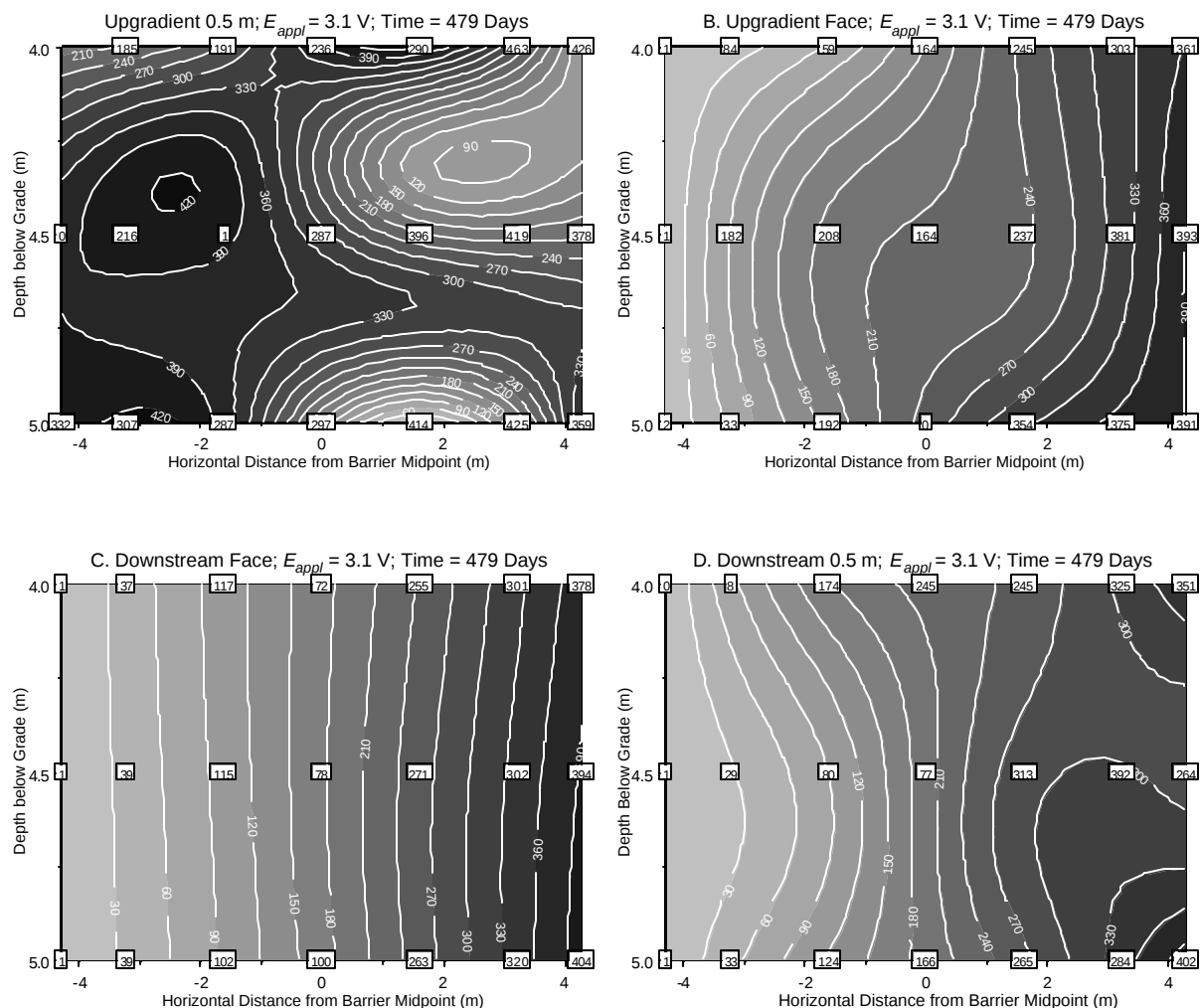
Figure E-3 - TCE concentration contour maps looking downgradient for E_{appl} = 3.1 V on day 479 at A. 0.5 upgradient of barrier, B. upgradient face of barrier, C. downstream face of barrier, and D. 0.5 m downgradient of barrier. Negative horizontal positions are to the west of the barrier midpoint, and positive positions are to the east. All concentrations are reported in mg/L. Boxes show measured concentrations at that location.
