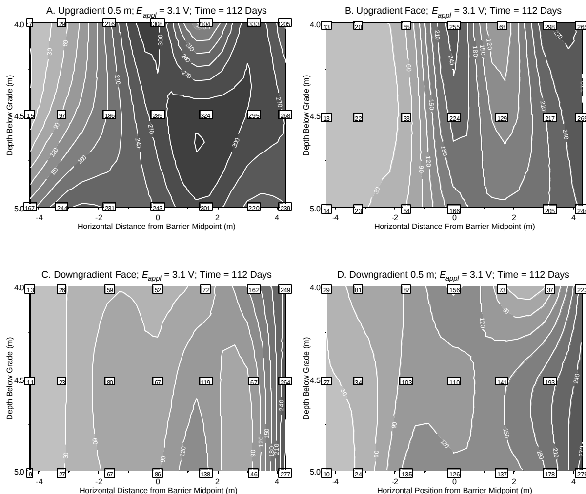
Figure E-2 - TCE concentration contour maps looking downgradient for E_{appl} = 3.1 V on day 112 at A. 0.5 upgradient of barrier, B. upgradient face of barrier, C. downgradient face of barrier, and D. 0.5 m downgradient of barrier. Negative horizontal positions are to the west of the barrier midpoint, and positive positions are to the east. All concentrations are reported in mg/L. Boxes show measured concentrations at that location.
