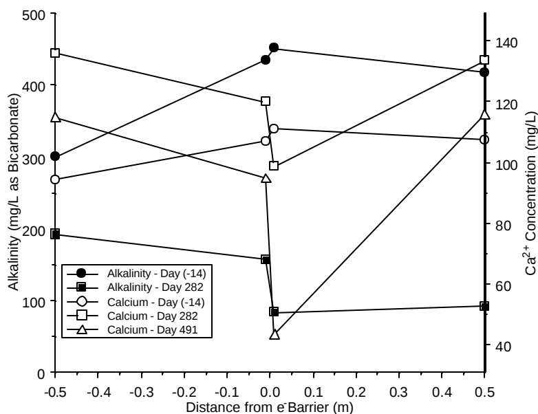
Figure 51. Alkalinity (as bicarbonate) and \text{Ca}^{2+} concentration measured along the transect parallel to groundwater flow through the e-barrier midpoint. Measurements were taken at 14 days prior to startup (alkalinity – closed circles, \text{Ca}^{2+} – open circles), day 282 (alkalinity – closed boxes, \text{Ca}^{2+} – open boxes), and day 491 (alkalinity – N/A, \text{Ca}^{2+} – open triangles). The e-barrier is located at 0 m and flow is from negative to positive distances.
