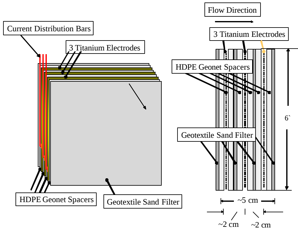
Figure 19. Composite panel detail
