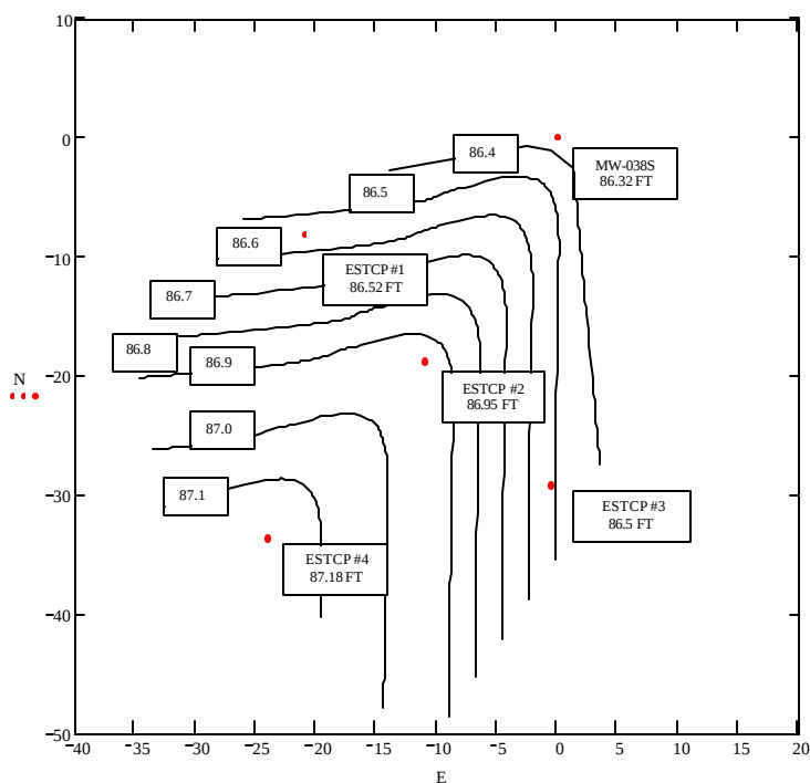
Figure 9. Potentiometric surface (11/18/2001)
