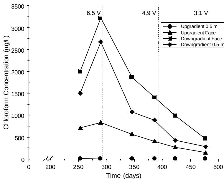
Figure 53. Average chloroform concentrations along the transect parallel to groundwater flow at the barrier midpoint. Values are arranged from 0.5 m upgradient of the barrier (circles), upgradient face of the barrier (triangles), downgradient face of the barrier (boxes), and 0.5 m downgradient of the barrier (diamonds). Power was applied to the barrier at day 0.
