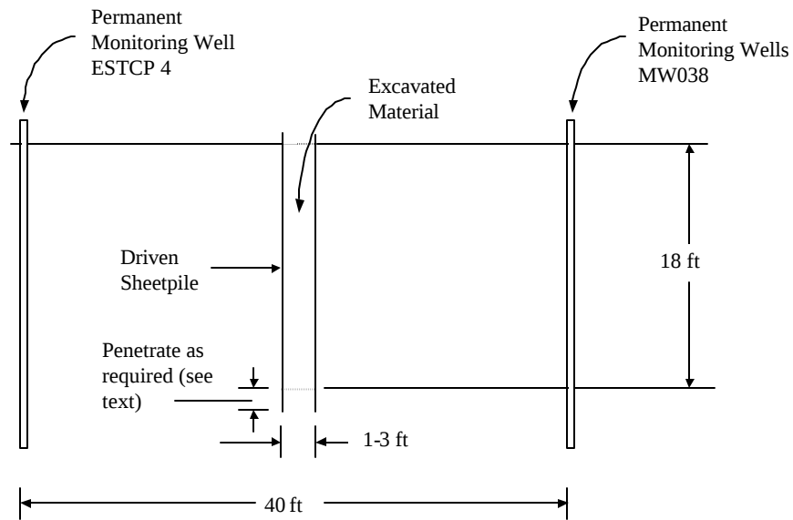
Figure 8 – Shoring to Grade Option
