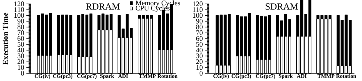
Figure 20: Execution times with various interleaving schemes.
