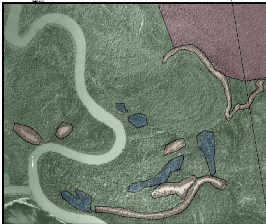
Figure 25. Example application of geomorphic mapping and aerial photography to develop a preliminary wetland classification for a proposed project area
