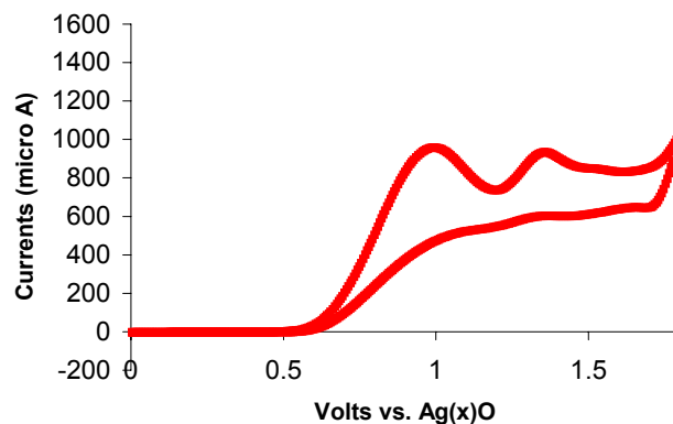
Figure 16. Voltammogram of Glassy Carbon (GC) Electrode in CH 3 OH/0.2 M LiClO 4 /100mM HMNAz/110mM TEA/110 mM NaNO 2
