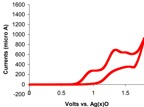
Figure 15. Voltammogram of Glassy Carbon (GC) Electrode in CH 3 OH/0.2 M LiClO 4 /100mM HMNAz/110mM TEA
