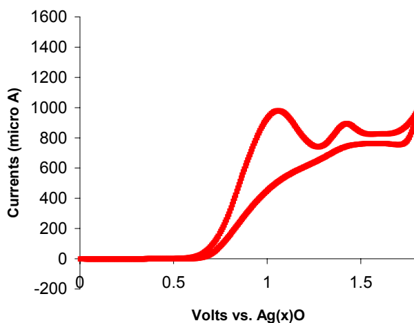
Figure 17. Voltammogram of Glassy Carbon (GC) Electrode in CH 3 OH/0.2 M LiClO 4 /100mM HMNAz/110mM NaOH/110 mM NaNO 2
