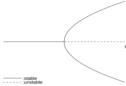
(c) Supercritical pitchfork bifurcation
