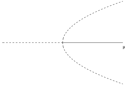
(b) Subcritical pitchfork bifurcation
