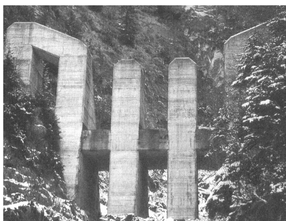
Figure 8. Stand-alone flow breakers (left) and flow breakers in debris dam (right) (from Fiebiger, 1997).
