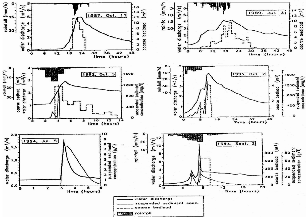
Figure 2. Rainfall hyetographs, streamflow hydrographs, and sediment transport rates for recorded floods (from Billi and others, 1998).
