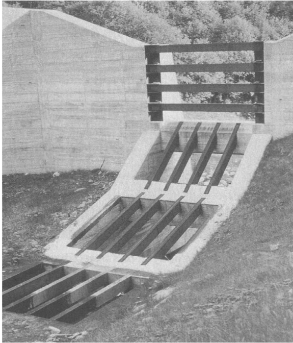
Figure 9. Debris-flow dam with a screen of steel beams (left, from Fiebigler, 1997) and open debris basin design (right, from VanDine, 1997).
