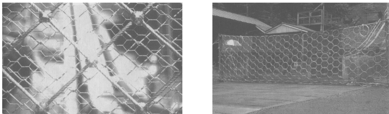
Figure 15. Flexible wire rope barriers with netting (left; models 1, 2, and 3) and with interlocking rings (right; model 4) (from DeNatale and others, 1997).
