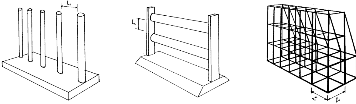
Figure 18. Column flow breaker (left), beam flow breaker (center), and grid flow breaker (right) (from Lin and others, 1997).
