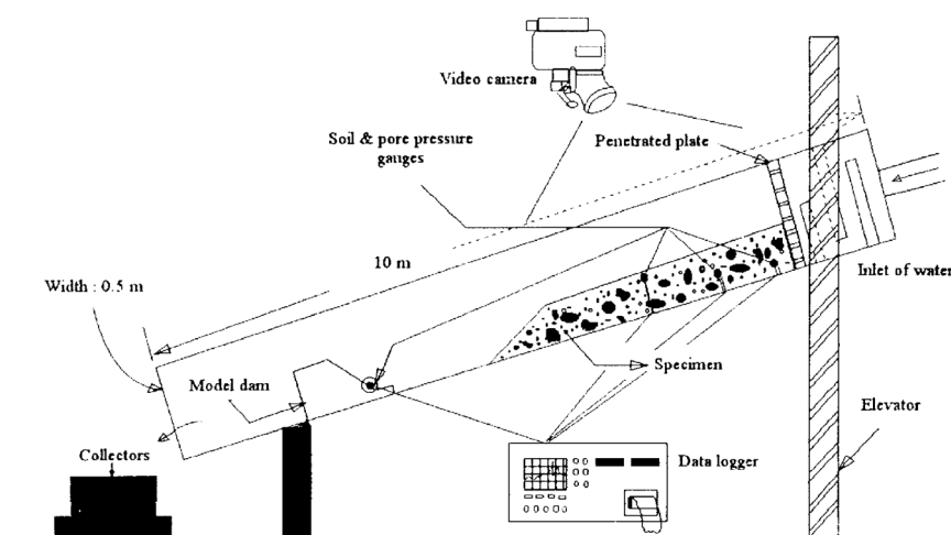
Figure 17. Flume test apparatus (from Chen and Ho, 1997).
