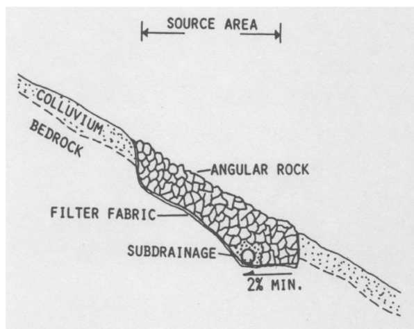
Figure 7. Riprap (left) on hillside in Pacifica, California, and riprap design recommendation (right) (from Baldwin and others, 1987).
