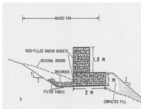
Figure 12. Gabion deflection wall, Tiburon, California (left), and design gabion deflection wall (right) (from Baldwin and others, 1987).
