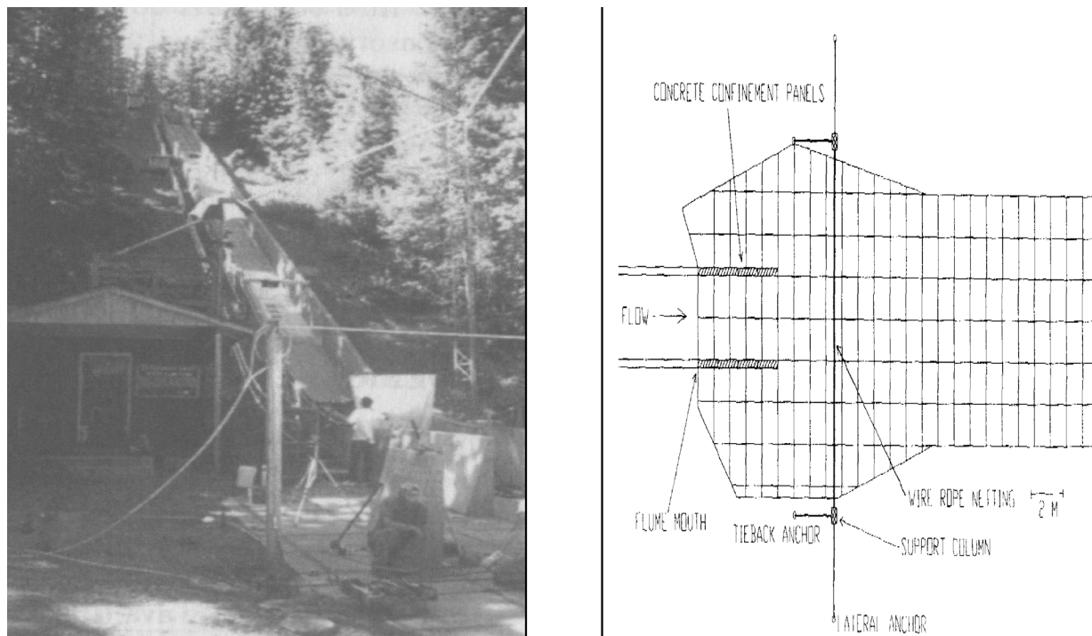
Figure 14. U.S. Geological Survey flume on Blue River at Blue Forest, Oregon (left), and schematic of the experiment to study the response of flexible wire rope barriers to debris-flow charges (right) (from DeNatale and others, 1997).
