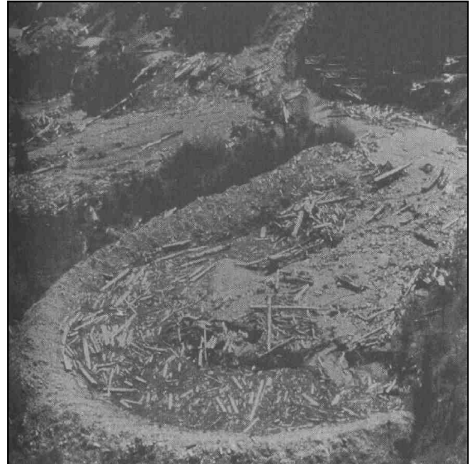
Figure 13. Terminal berm schematic (left) and terminal berm on Cypre Creek in British Columbia (right) (from VanDine, 1997).
