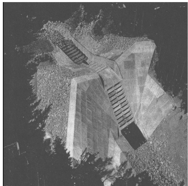
Figure 10. Closed debris basin schematic (left) and closed debris basin on Harvey Creek in British Columbia (right) (from VanDine, 1997).
