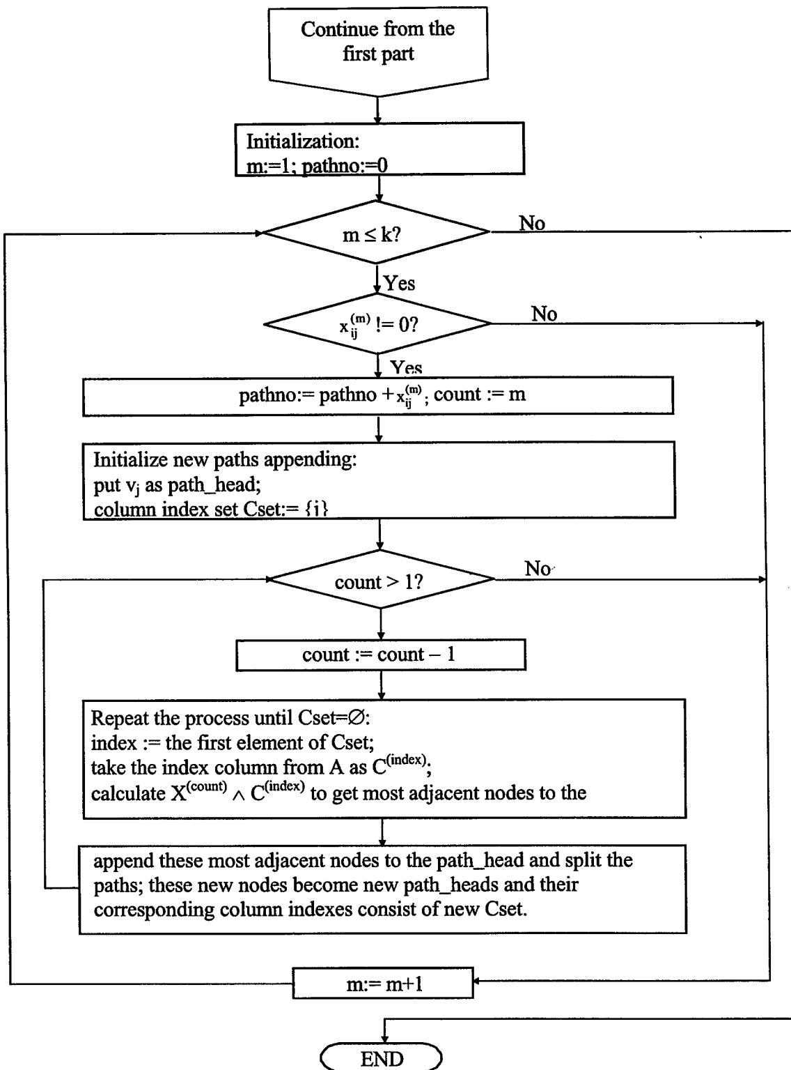
Figure 3.3.5. Path-Searching Algorithm (Part II)
