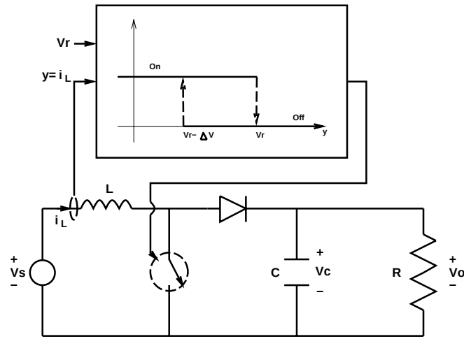
Figure 4: System diagram for a boost converter under hysteresis control
