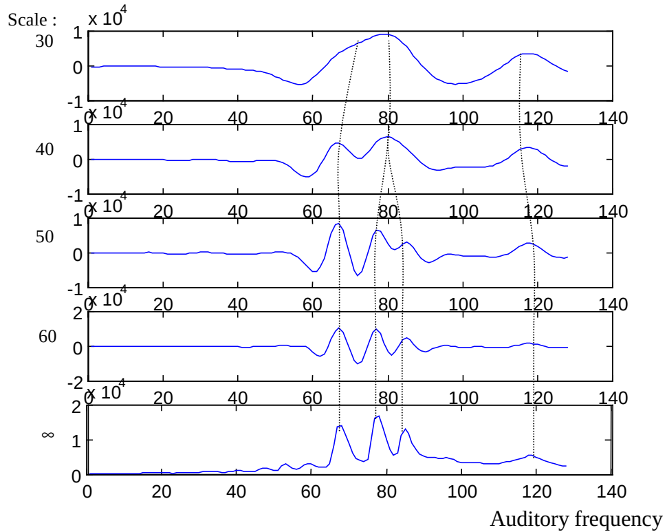
Figure 2.6. Cortical representation at different scales. From top to bottom are scales 30, 40, 50, 60, and ' \infty '. Where ' \infty ' means raw spectrum from auditory module.
