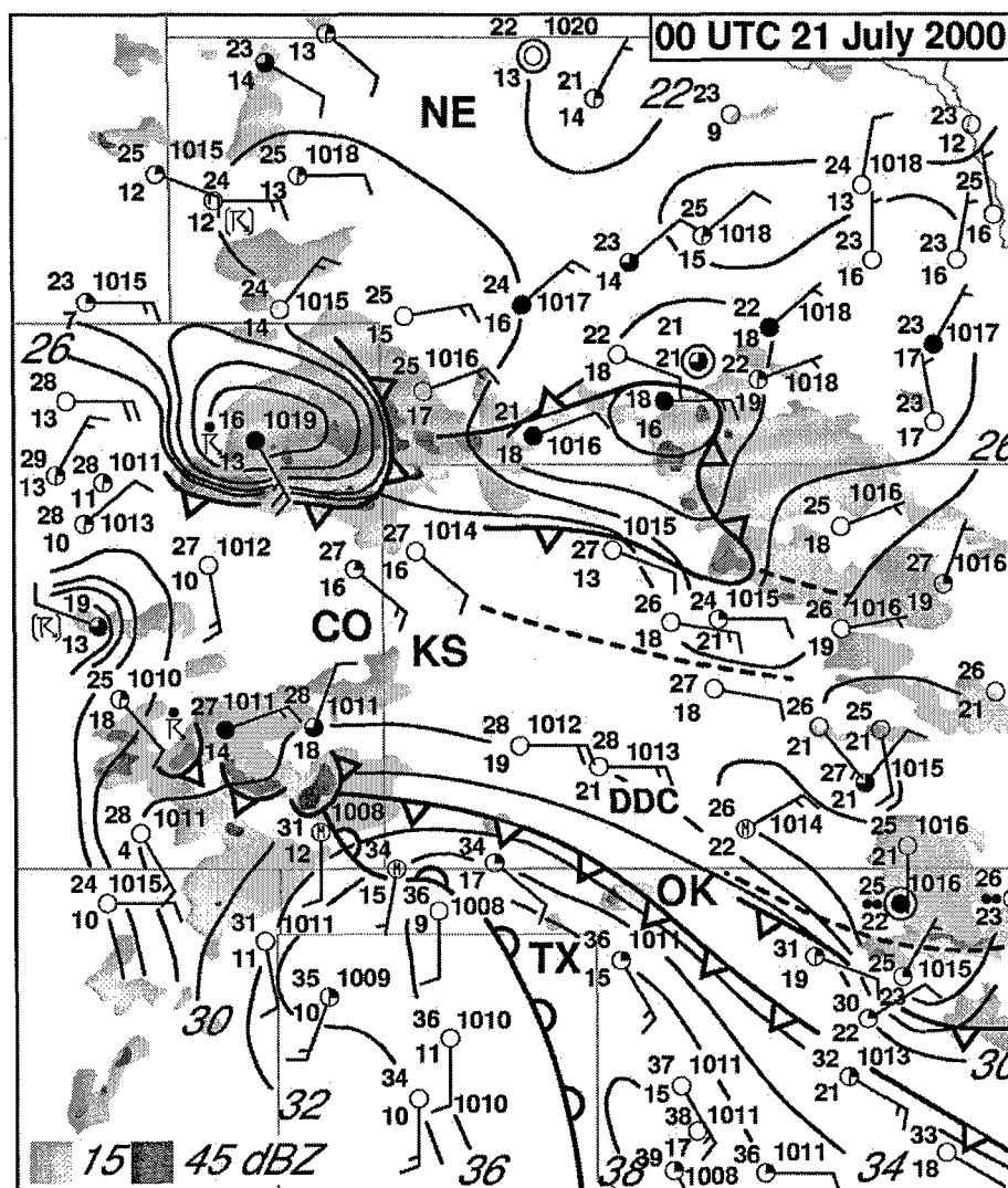
Figure 16. Surface analysis at 00 UTC on 21 July 2000, the starting time for the forecast period. Conventional station model format includes temperature ( ^{\circ}\text{C} ) over dewpoint ( ^{\circ}\text{C} ), mean sea level pressure (mb) at upper right, and wind barb (full barb = 5 \text{ m s}^{-1} , half barb = 2.5 \text{ m s}^{-1} ). Instantaneous base radar reflectivity is shown by gray fill. The site of Dodge City sounding discussed in the text is indicated by "DDC."
