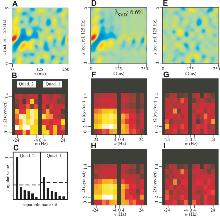
Figure 7: Approximating the \text{MTF}_{\text{ST}} with the SVD. A, B: The original STRF measurement and the corresponding \text{MTF}_{\text{ST}} magnitude (first two quadrants). C: The singular values (bars) and thresholds (dashed lines) of the first two quadrants of the \text{MTF}_{\text{ST}} . D, E: The quadrant-separable approximation of the STRF and the remainder. F, G: The \text{MTF}_{\text{ST}} magnitude from the quadrant-separable approximation, and the Fourier Transform of the remainder. H, I: The \text{MTF}_{\text{ST}} magnitude from the \text{rank-2} approximation (from Figure 6I), and the Fourier Transform of the remainder (from 6J)
