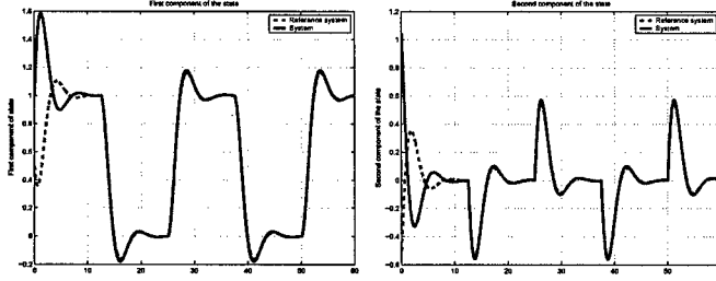
Fig. 1 Tracking performance.
