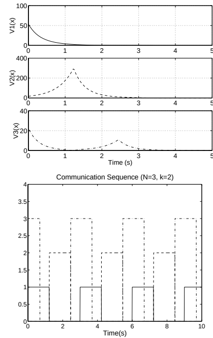
Figure 2: Top: Time evolution of the Lyapunov function of each system. Bottom: The corresponding communication sequence.
