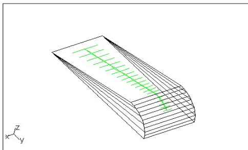
Figure 8. Shifted Log-Periodic Antenna
