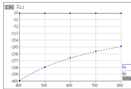
Figure 15. Input Impedance
