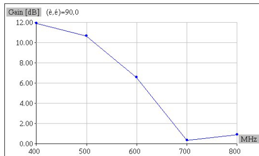
Figure 9. Gain at 0° elevation
