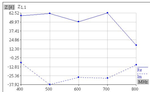
Figure 7. Input impedance
