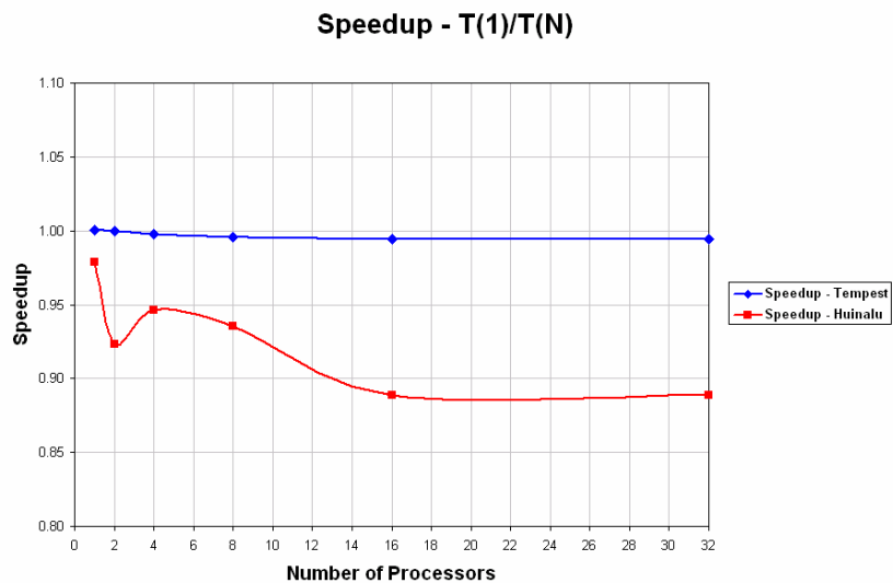
Figure 2 – Speedup Results for Frequency Parallelization
