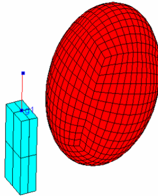
Figure 1 – Cell Phone Alongside a Dielectric Ovoid
