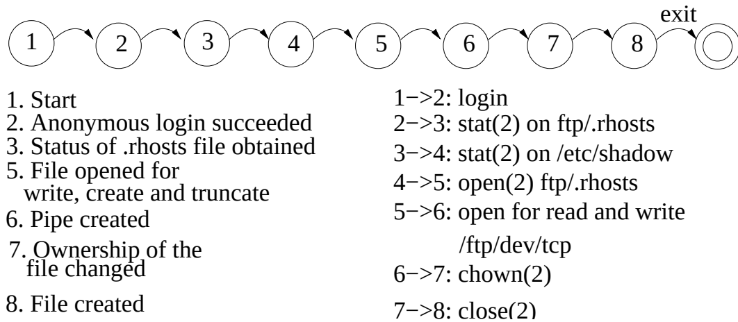
Figure 3.11: Ftp-write attack - create file phase.
