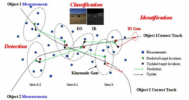
Figure 3. Data Association using ID and Position Measurements.
