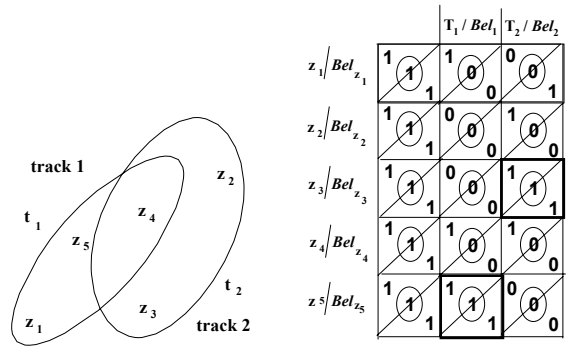
Figure 6. Tracking and Classification Joint Association
