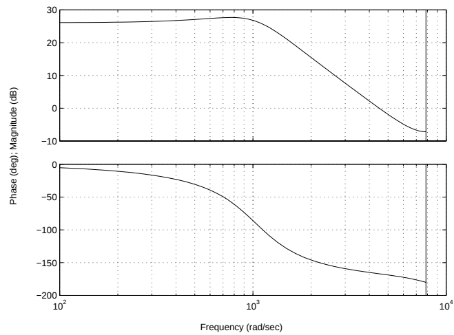
Figure 7: Duty-ratio-to-output frequency response for Example 1
