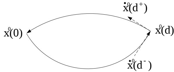
Figure 3: A typical periodic solution x^0(t) of a PWM converter in state space
