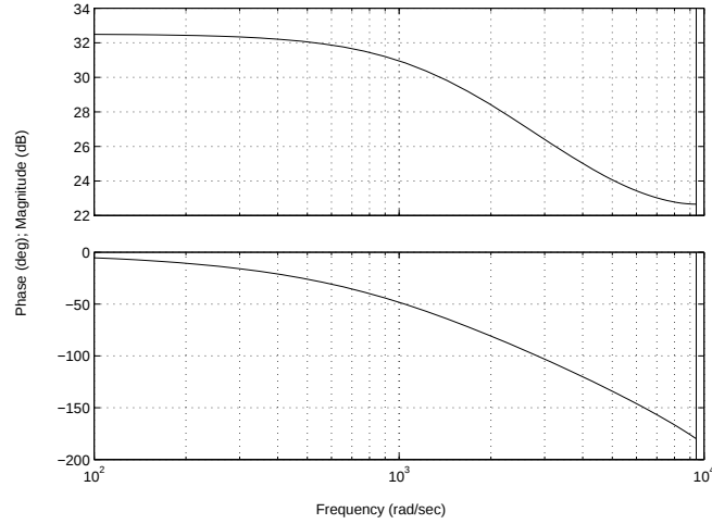
Figure 9: Duty-ratio-to-output frequency response for Example 2
