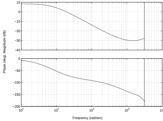
Figure 12: Duty-ratio-to-output frequency response for Example 4
