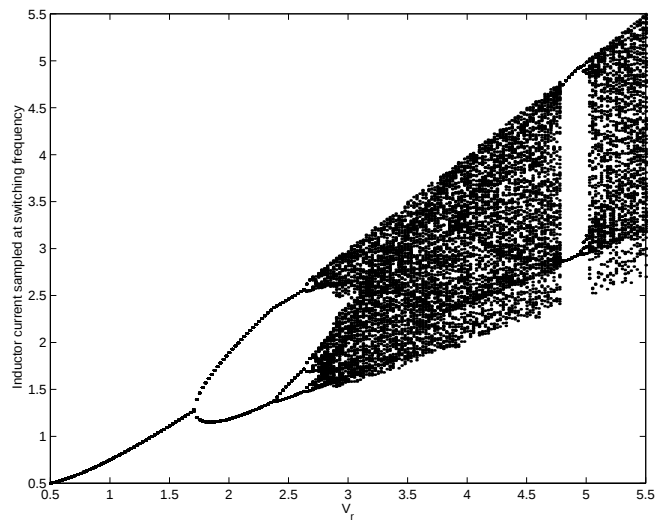
Figure 12: Bifurcation diagram of the circuit in Fig. 11
