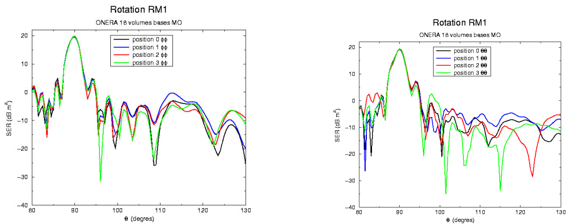
Figure 5 : Computed RCS modulations at 16 Ghz, \alpha = 0^\circ , \alpha = 5,625^\circ , \alpha = 11,250^\circ , \alpha = 16,875^\circ
