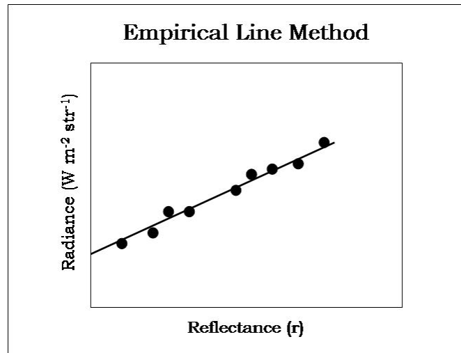
Figure 2.1 ELM Representation
