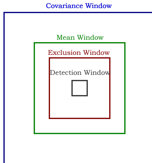
Figure 3.14 Four-Part Sliding Window Implementation
