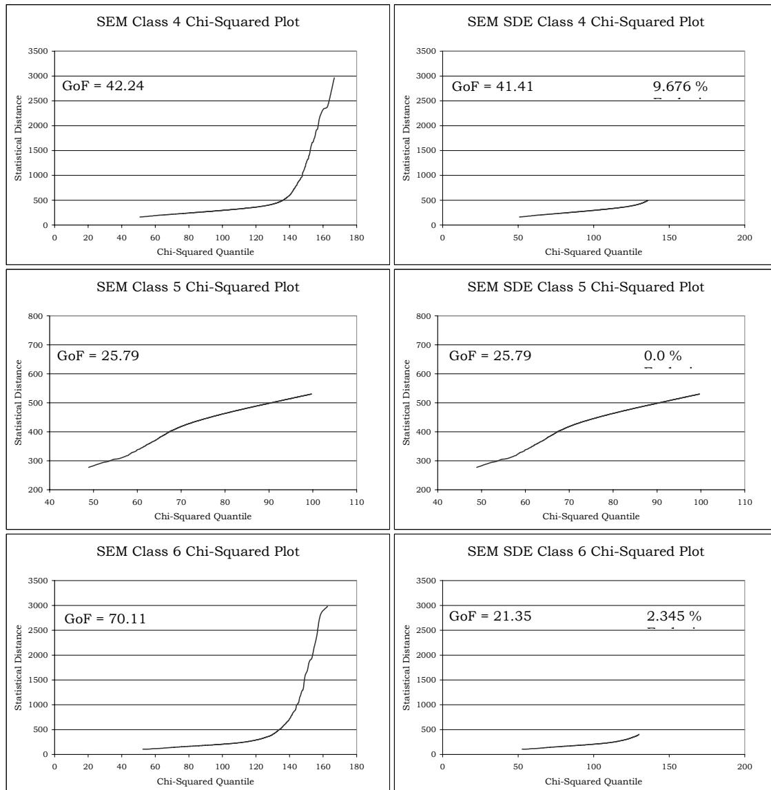
Figure A.18 SDE Chi-Squared Example for SEM Classes 4 – 6
