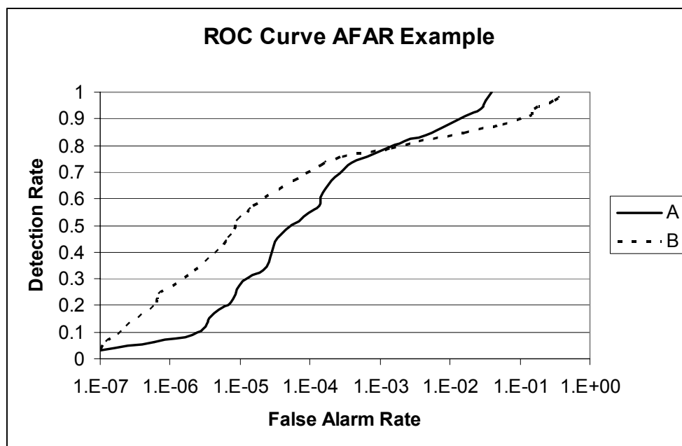
Figure 3.28 Example ROC Curve Illustrating the Need for a Partial AFAR
