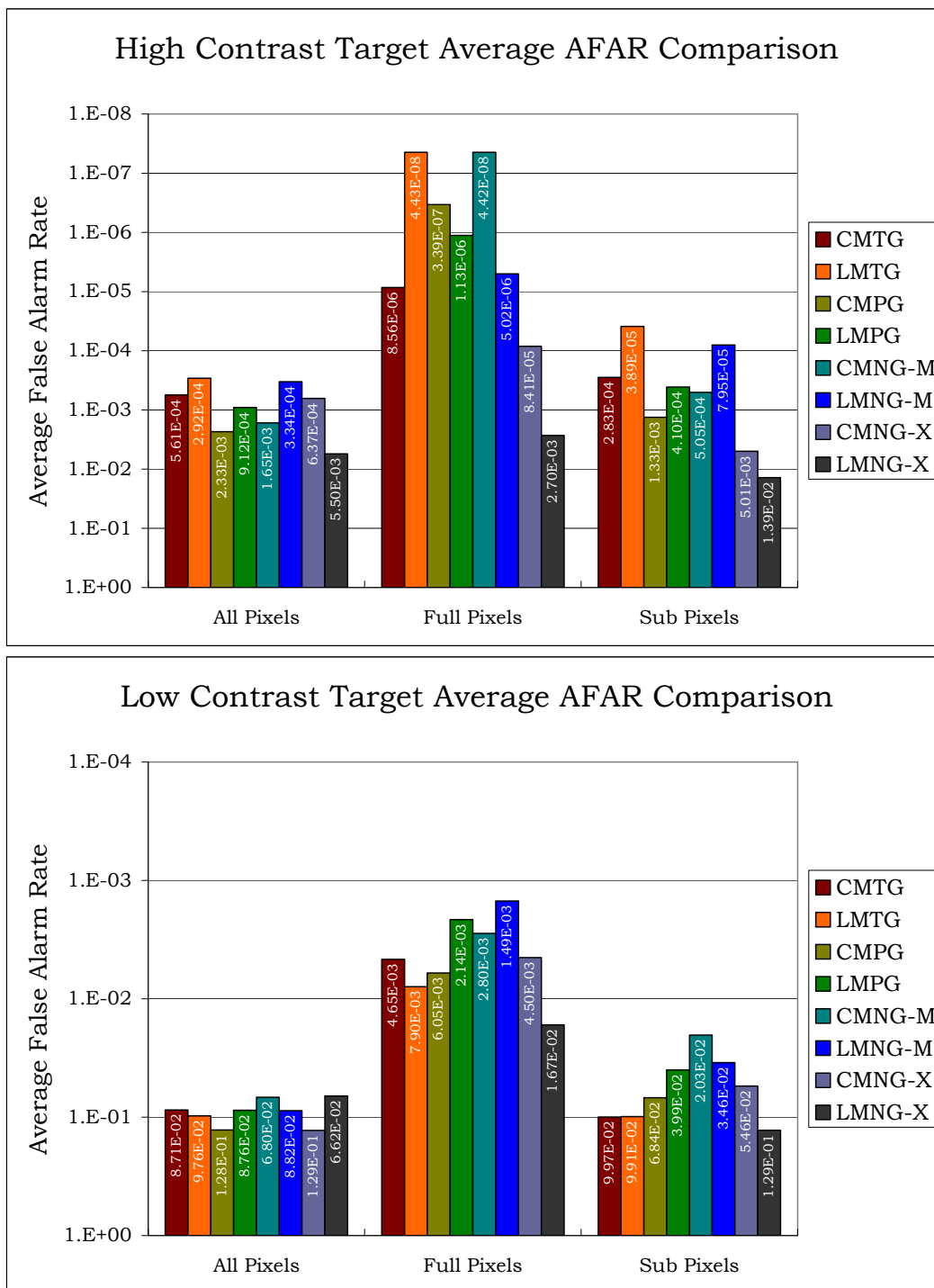
Figure 4.16 Run05 Pre-Clustering Summary AFAR Plots
