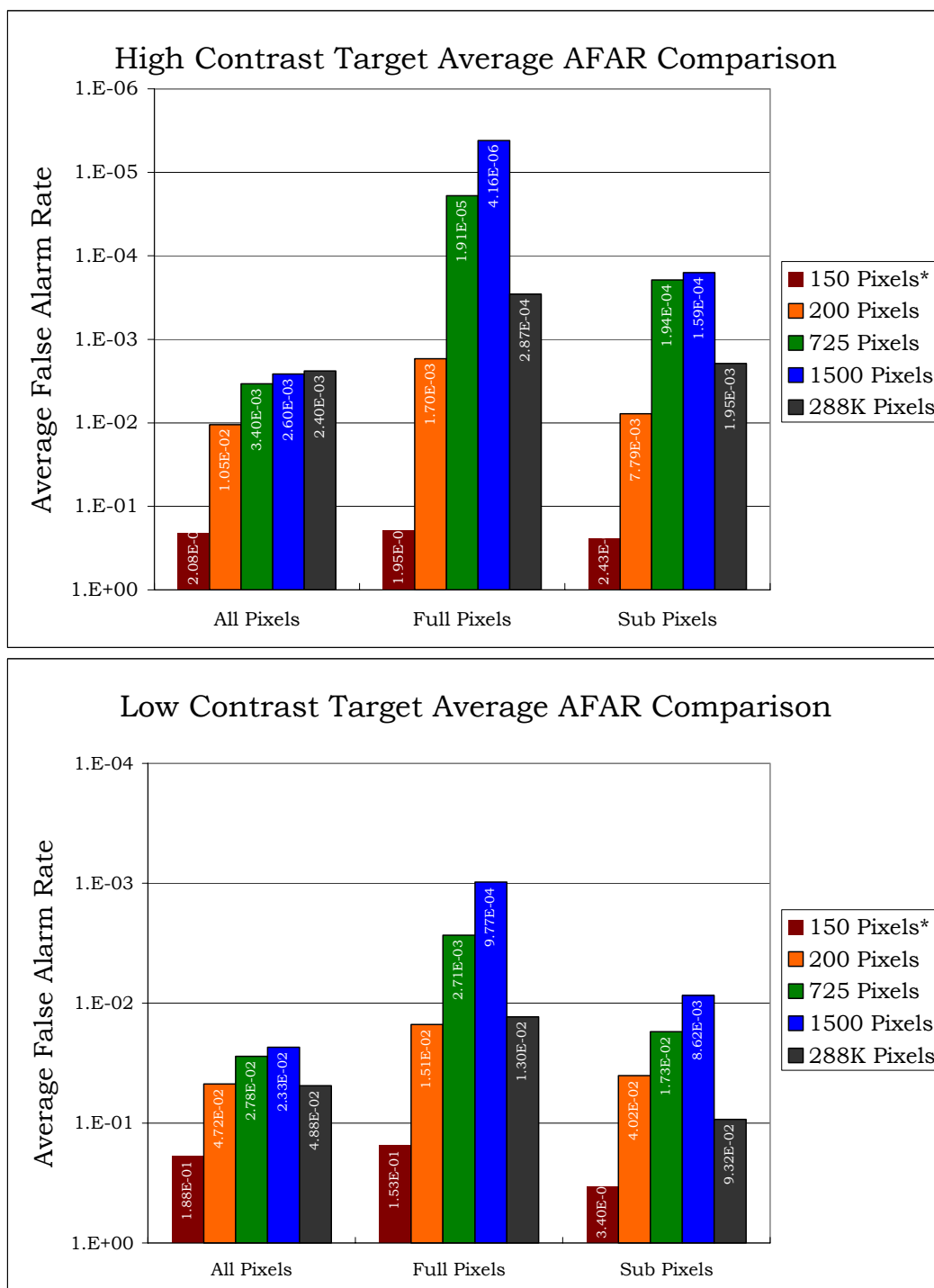
Figure 4.7 Run03 RX Sliding Window Summary AFAR Plots
