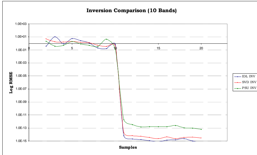
Figure 3.12 Ten Band Comparison of Inversion Techniques
