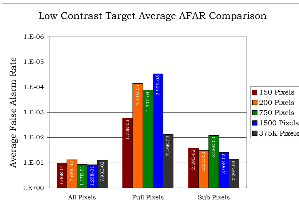
Figure 4.6 Run05 RX Sliding Window Summary AFAR Plots
