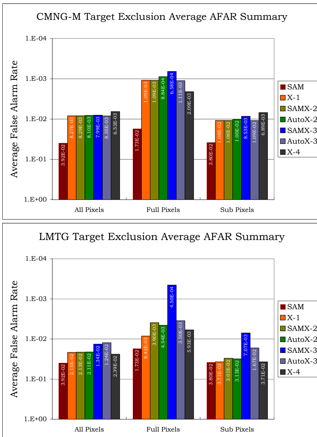
Figure 4.18 Pre-Clustering Target Influence Summary AFAR Plots
