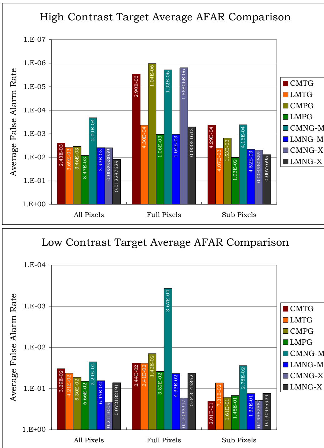
Figure 4.17 Run03 Pre-Clustering Summary AFAR Plots
