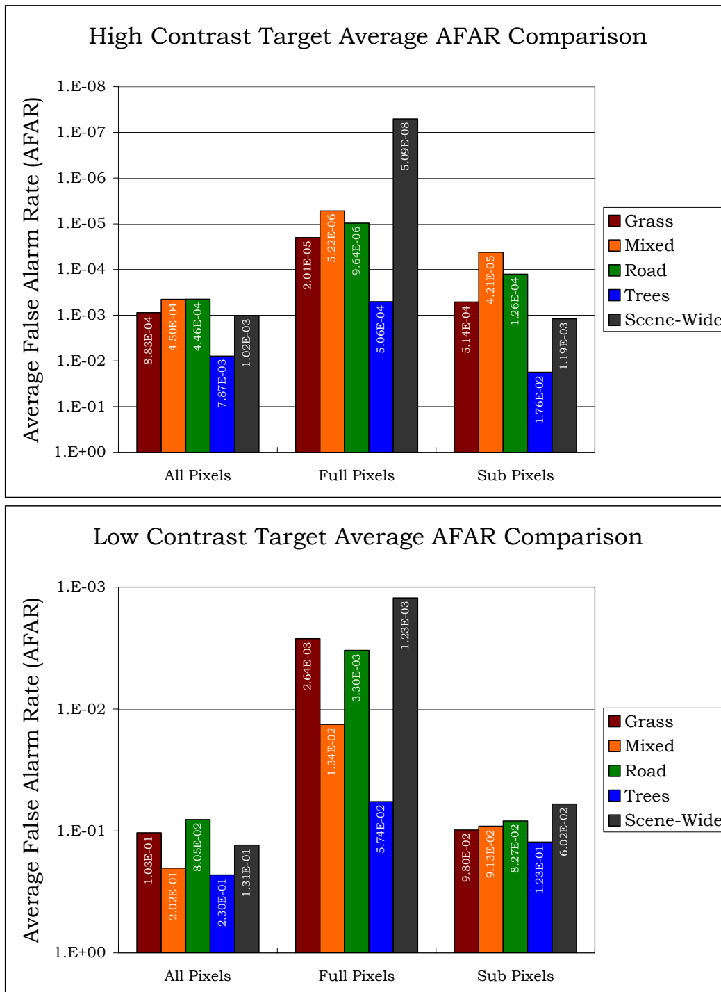
Figure 4.1 Run05 Target Approach Summary AFAR Plots
