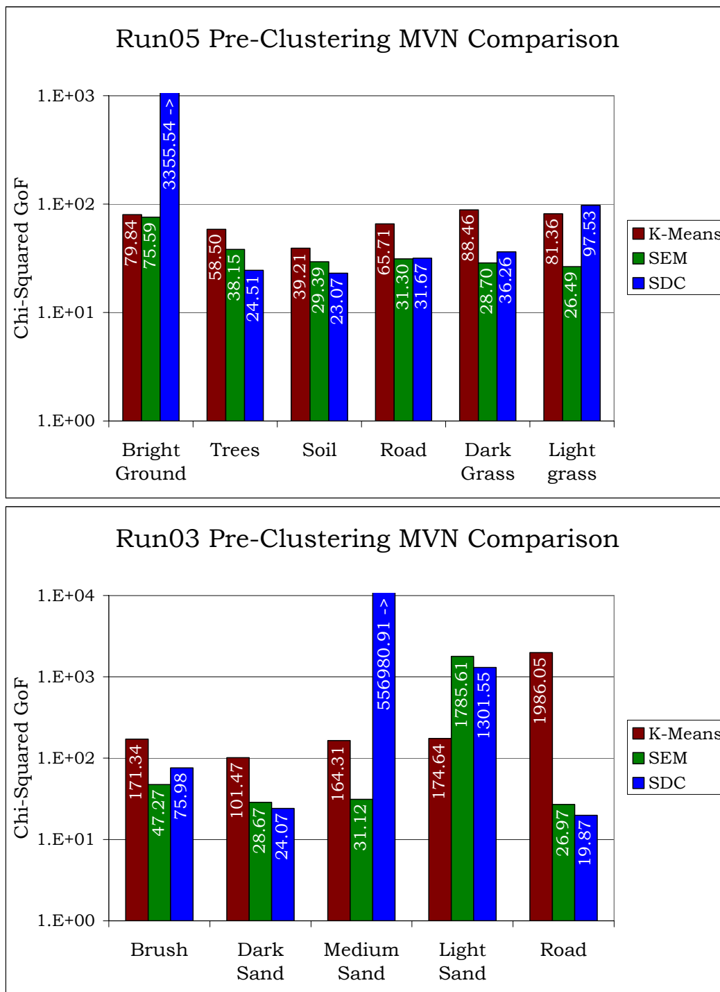
Figure 4.15 Run05 and Run03 Pre-Clustering MVN
