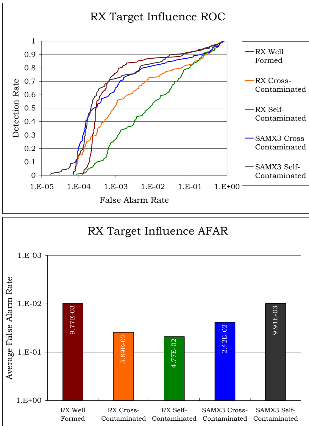
Figure 4.10 RX Sliding Window Target Influence Example
