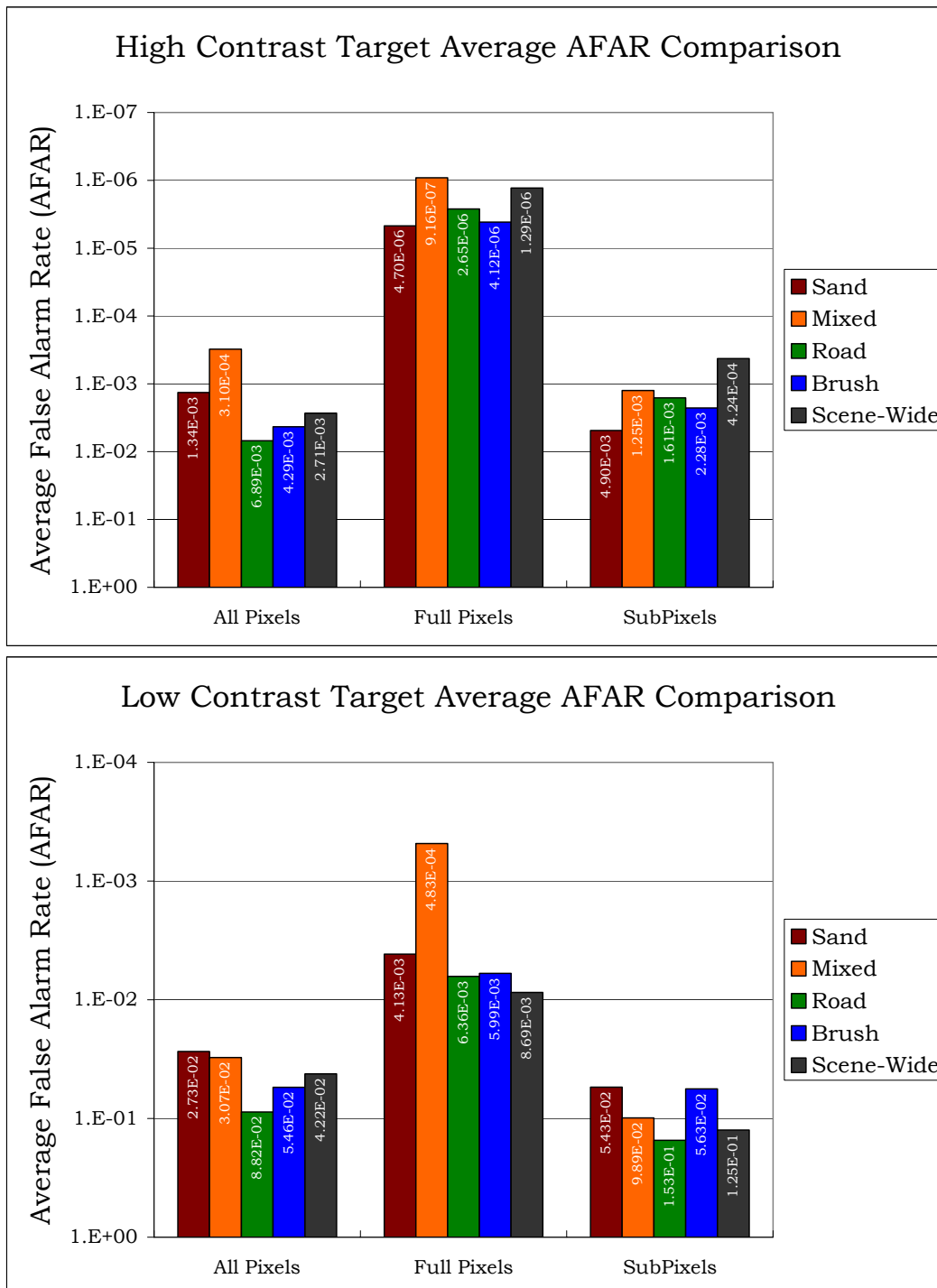
Figure 4.2 Run03 Target Approach Summary AFAR Plots
