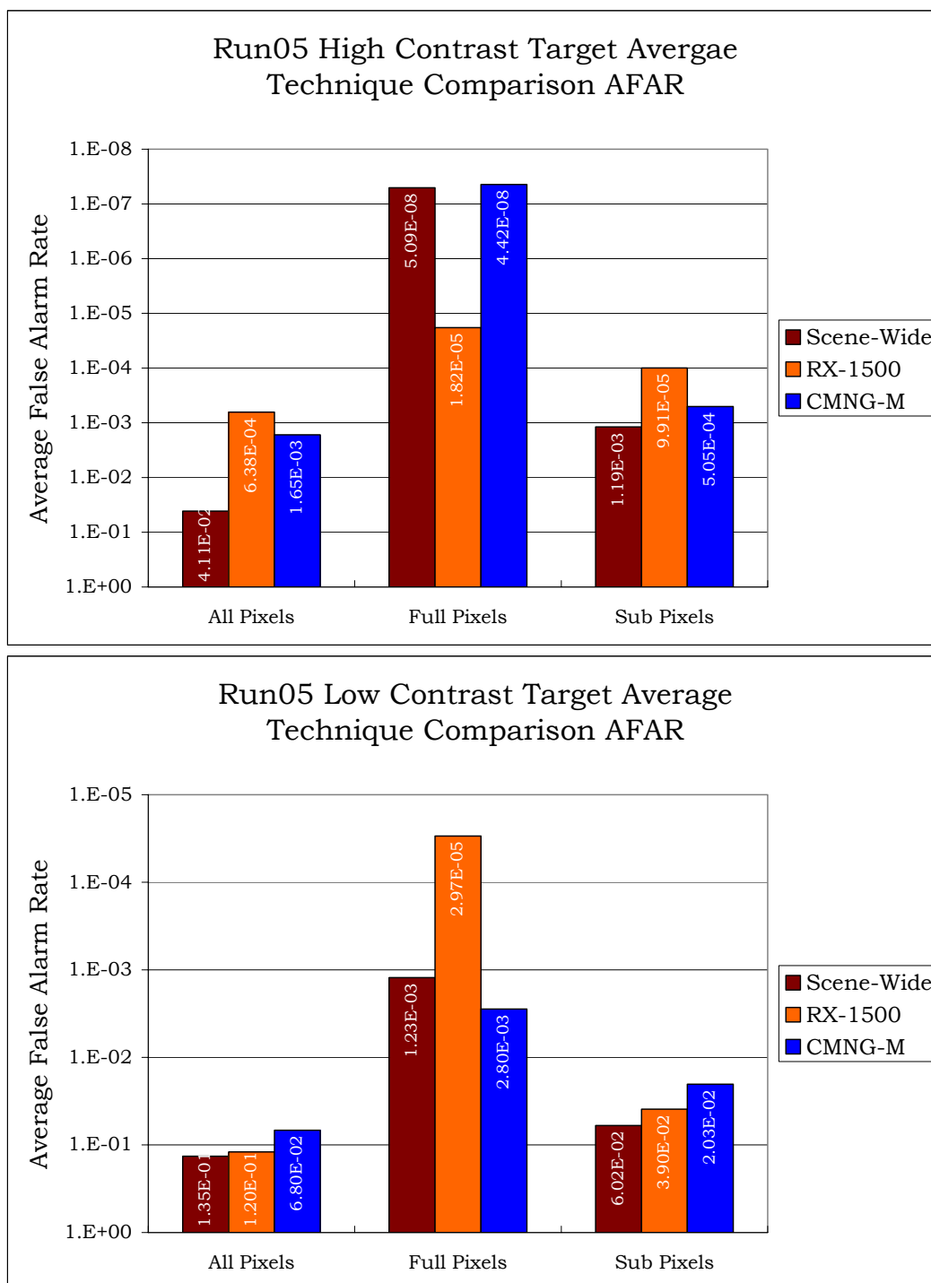
Figure 4.20 Run05 High and Low Contrast AFAR Final Comparison
