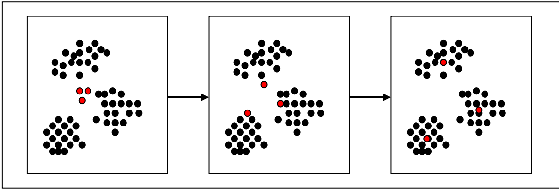
Figure 2.2 K-Means Classification
