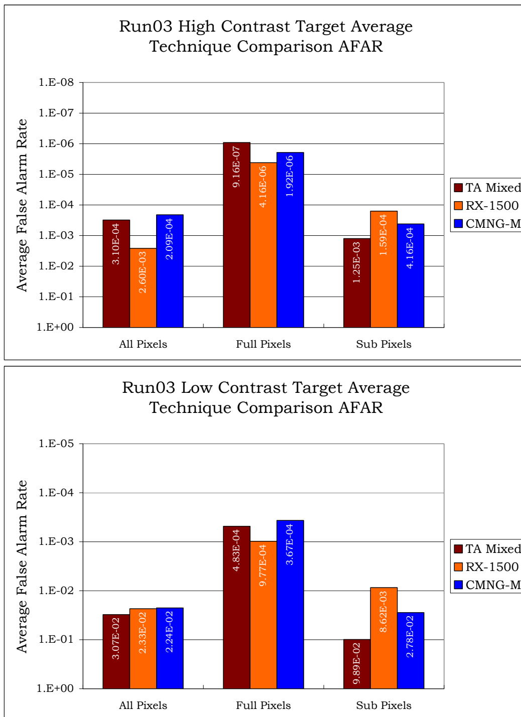
Figure 4.21 Run03 High and Low Contrast AFAR Final Comparison
