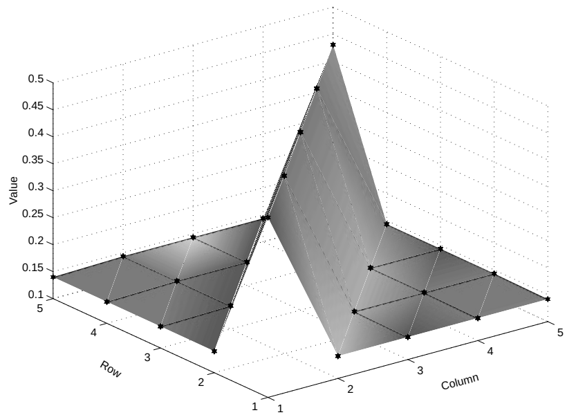
Figure 4.11: Observation matrix (B) for Day 4
