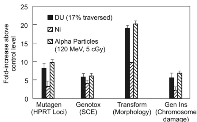
Figure 1. A comparison of the mutagenicity, genotoxicity, neoplastic transformation, and genomic instability resulting from cellular exposure to DU, NI, or, alpha particles is shown. Results are from greater than three experiments per endpoint and greater than three replicates were used per experiment. Cell culture (human osteoblast cells HOS), neoplastic transformation, genotoxicity, mutagenicity, and genomic instability methods have all been previously described [Miller 1998a, 1999, 20002a, 2002b, 2001, 2002, 2003, 2004]. DU dioxide 925 \mu\text{g}/\text{ml} ; 24 hrs) and crystalline nickel (25 \mu\text{g}/\text{ml} , 24 hrs) were used. The microdosimetry demonstrated that during DU exposure, 17% of the cell nuclei were traversed by an alpha particle (21 \mu\text{Gy}/\text{nuclei} ). During alpha particle beam exposure 100 % of cells were traversed (24 \mu\text{Gy}/\text{nuclei} ). Significance was determined by ANOVA; significance set at P < 0.05 . For all endpoints there was a significant increase above background; there was no significant difference between alpha particle exposure and DU.
