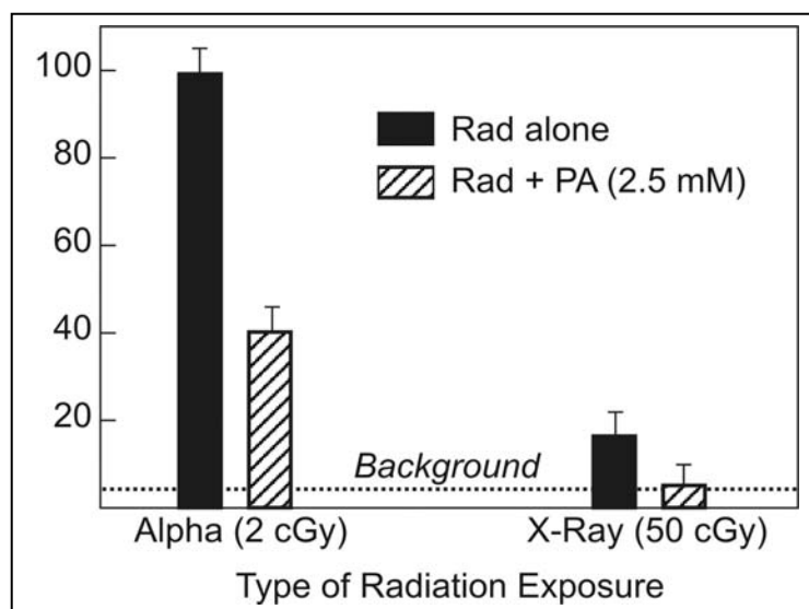
Figure 3. Modulation of Neoplastic cell transformation by PA (2.5 mM 6 weeks) after exposure to either alpha particles (2 cGy, 120 MeV broad beam) or X-rays (50 cGy 150 MeV) is demonstrated in this figure. HOS cells were irradiated to induce transformation. Cell culture, neoplastic transformation, and alpha radiation (Columbia University, Radiological Research Accelerator Facility (RARAF)) have been previously described [Miller 1998a, 1999, 2001, 2004]. Three experiments with three replicates per point were done. Significance was determined by ANOVA; significance set at P < 0.05 . There was a significant difference between alpha-induced and X-ray induced transformation and control; PA treatment caused a significant reduction in transformation.
