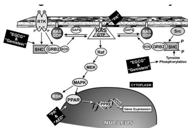
Figure 2: Signal Transduction Pathway
