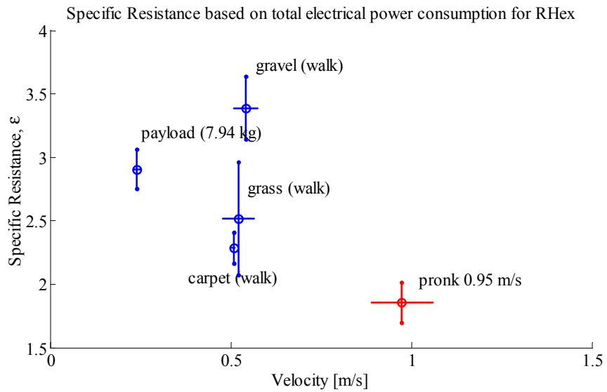
Figure 6: RHex specific resistance during walking and pronking
