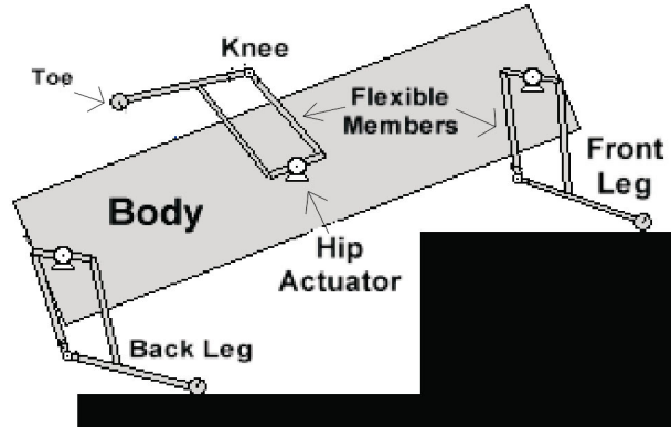
Figure 3. Main Components
