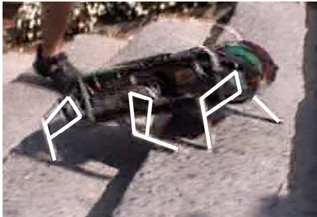
Figure 4. Dynamic tripod gait on shallow stairs – legs highlighted for clarity
