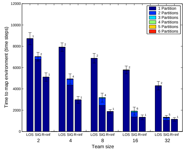
Fig. 7. Mean number of time steps to map dense environment versus team size , broken down by number of partitions in the network. “LOS” indicates the line of sight coordination method, “SIG” denotes the signal strength based coordination method, and “R=inf” denotes the case where communication range is assumed to be infinite and signal strength based coordination is used. The error bars represent one standard deviation, and the numbers to the upper left of each bar indicate the maximum number of network partitions present at one time in any of the 25 trials represented by the bar.
