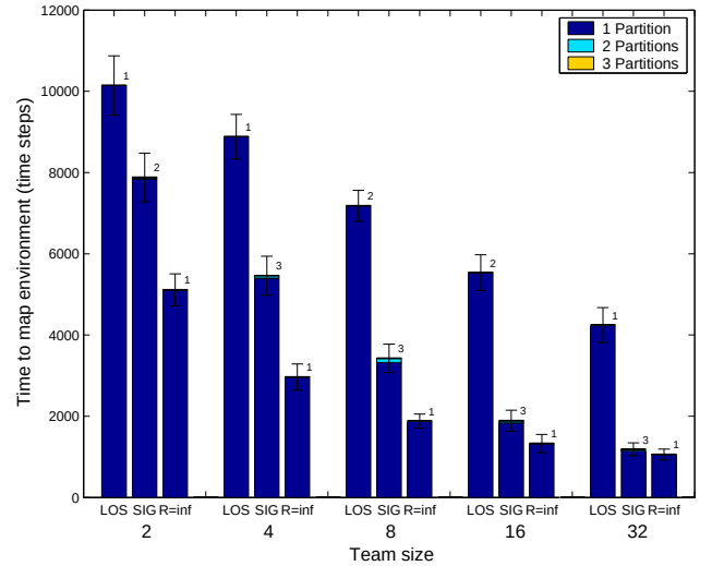
Fig. 6. Mean number of time steps to map sparse environment versus team size , broken down by number of partitions in the network. “LOS” indicates the line of sight coordination method, “SIG” denotes the signal strength based coordination method, and “R=inf” denotes the case where communication range is assumed to be infinite and signal strength based coordination is used. The error bars represent one standard deviation, and the numbers to the upper left of each bar indicate the maximum number of network partitions present at one time in any of the 25 trials represented by the bar.
