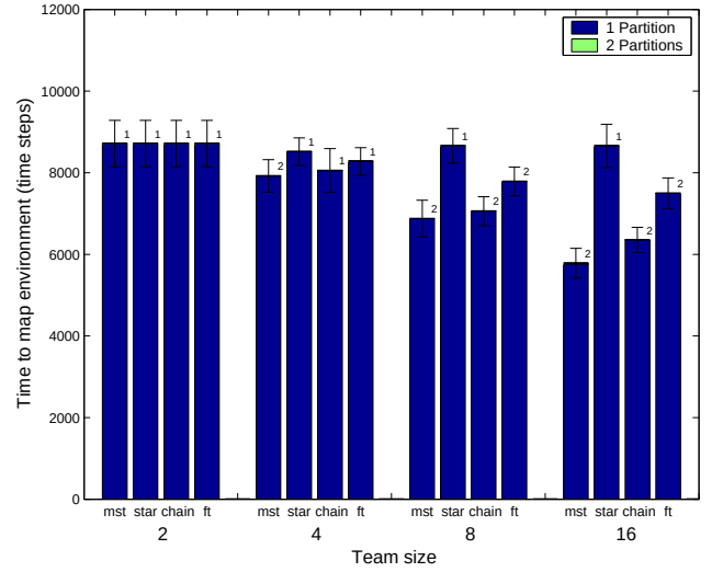
Fig. 16. Performance of topologies using line of sight coordination in the dense environment: A comparison the “minimum spanning tree” (mst), “star”, “chain”, and “fixed tree” (ft) topologies using the line of sight method in the dense environment. The error bars represent one standard deviation, and the numbers to the upper left of each bar indicate the maximum number of network partitions present at one time in any of the 25 trials represented by the bar.
