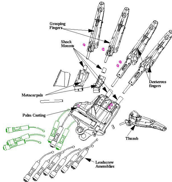
Figure 2. Robonaut hand parts
