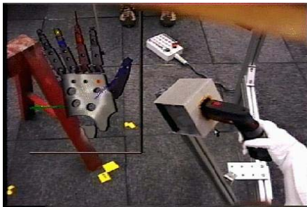
Figure 7. Robonaut gloved hand grasping drill in holster
