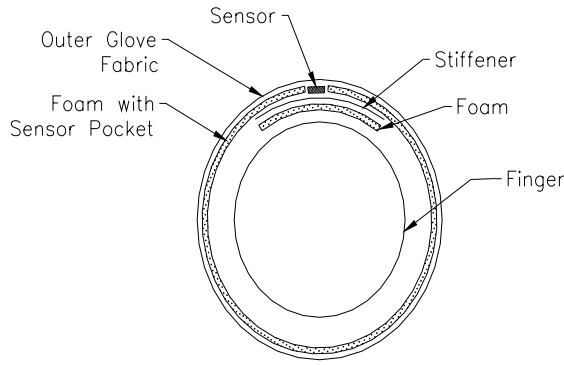
Figure 6. Interlink sensor packaging (cross-section) not-to-scale
