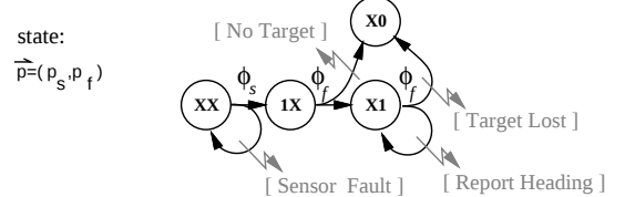
SACCAD-FOVEATE B-Pgm:
