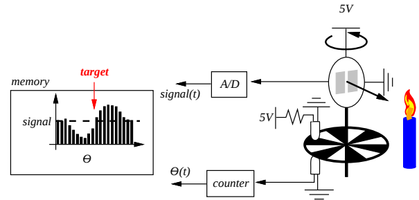
Figure 4. Pyroelectric sensor.
