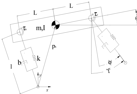
Figure 2: Scout II model
