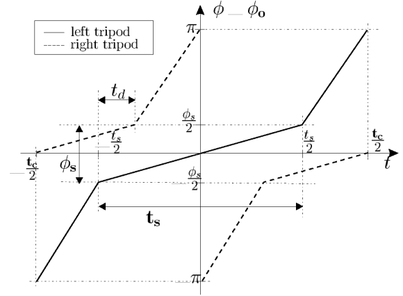
Figure 9: Motion profiles for left and right tripods.
