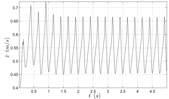
Figure 10: Simulation of forward body velocity.
