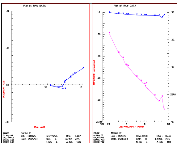
Figure 3.06. Complex resistivity (CR) spectrum corresponding to a dipole centered over a 3” steel sphere immersed in Tucson tap water.
