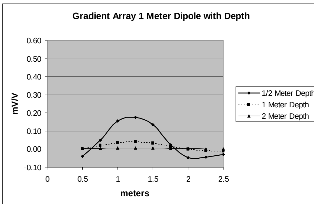
Figure 3.16: Target range for 10 m AB, 1 m MN Gradient Array in deep water
