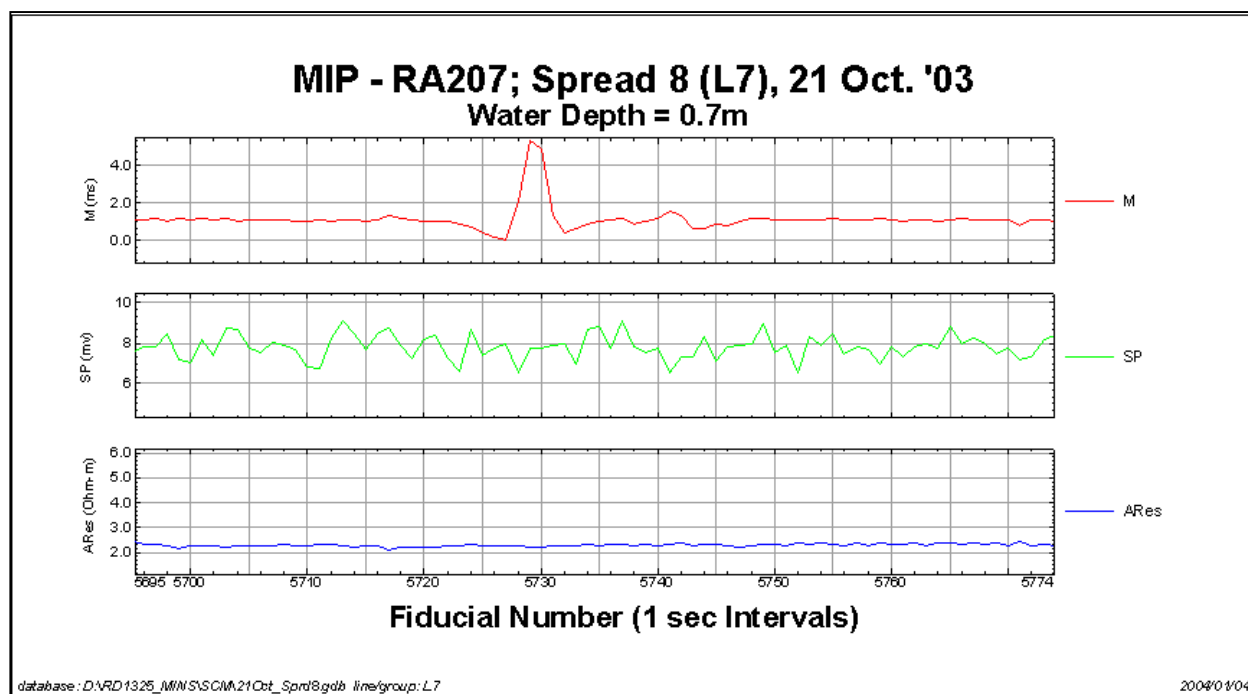
Figure 5.06: Center-line profile crossing target RA207. Sample rate = 1 sample/sec. RA207 is located at fid number 5729. A second anomaly (fid 5742) a much smaller amplitude correlates with RA208.
