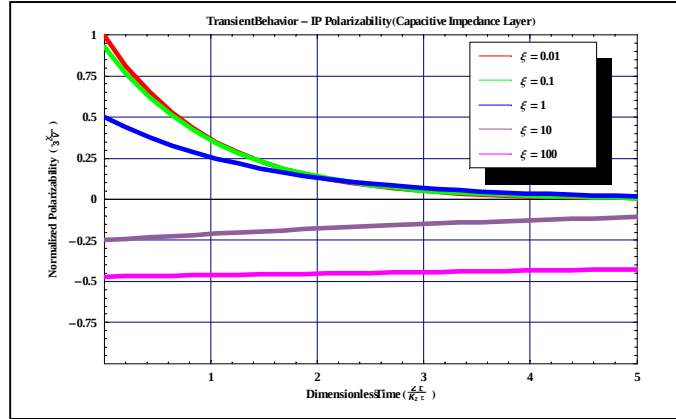
Figure 2.04: Parametric plot showing relative time-domain IP polarizability as a function of time with \xi as the parameter. The results are based on a capacitive model of Faradaic electrode impedance.
