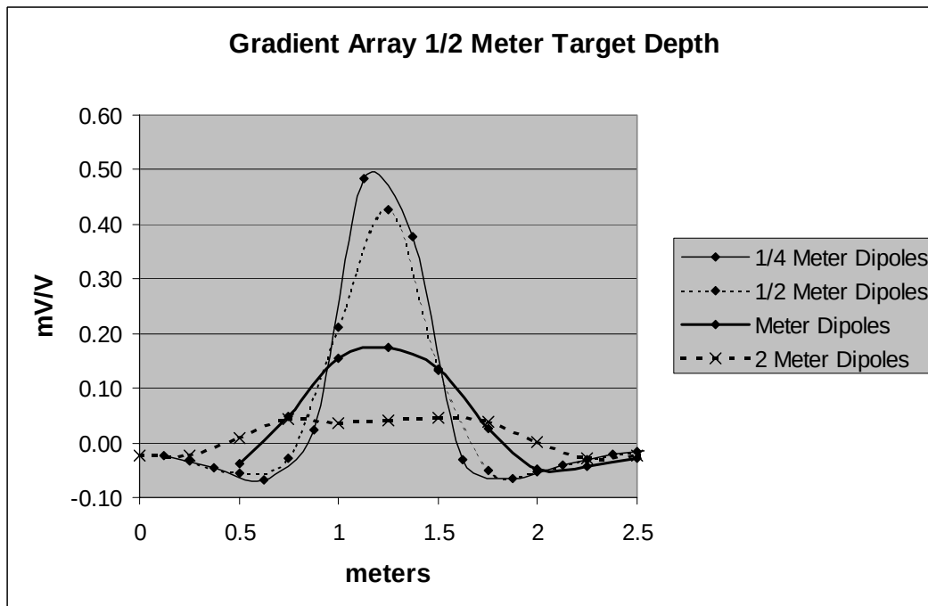
Figure 3.15: Dipole size comparisons for 5 m AB (1/4 and 1/2 m MN) and 10 m AB (1 meter MN) gradient arrays in fresh water.
