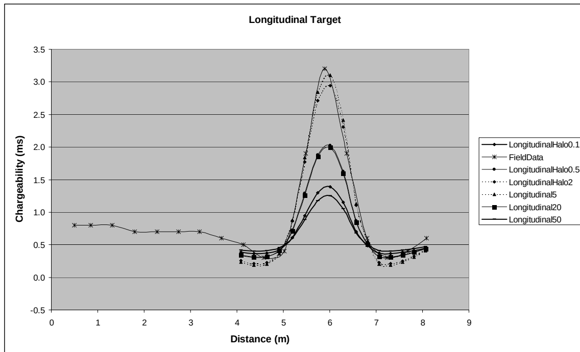
Figure 3.13: Calibration of model results to the longitudinal target field response by varying the resistivity of the resistive shell.
