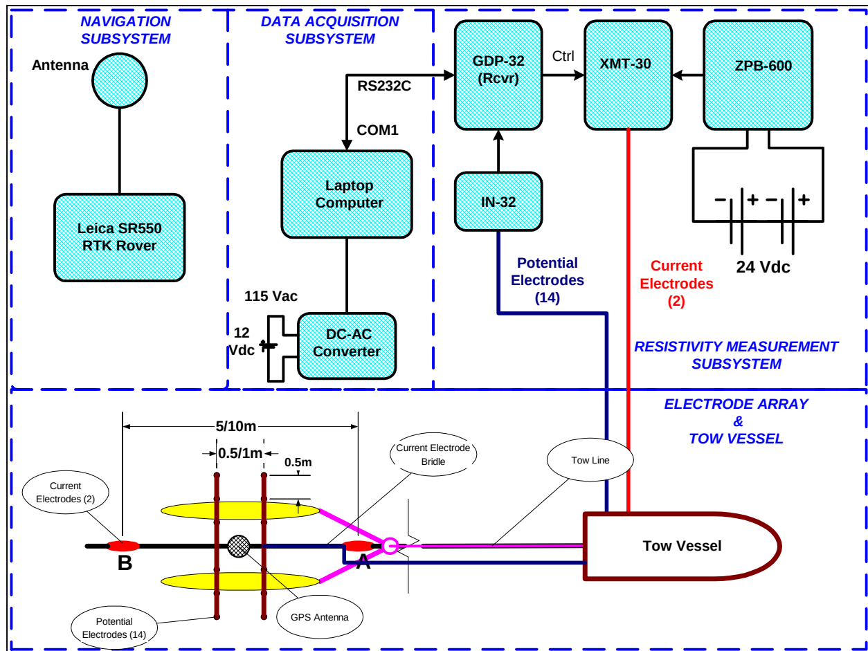
Figure 4.01: Block diagram showing major functional elements of the system assembled for full-scale field
