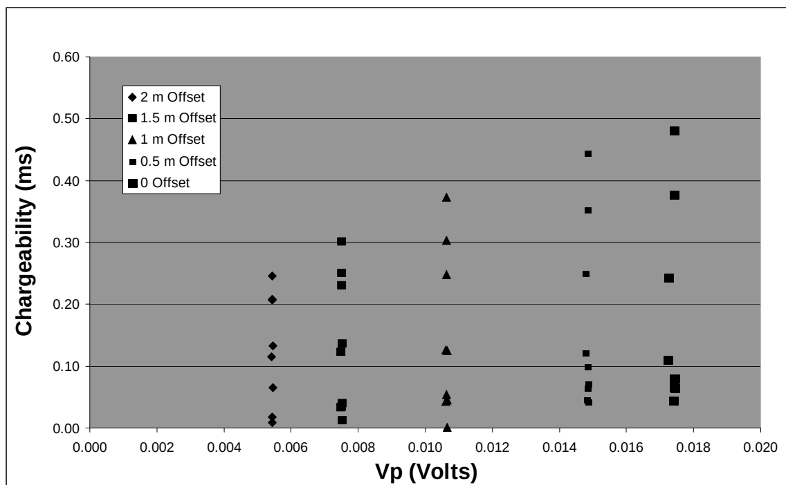
Figure 3.20: IP response versus primary field voltage for a 5m AB offset gradient array. The parameter is the lateral offset of the receiver dipole from AB.
