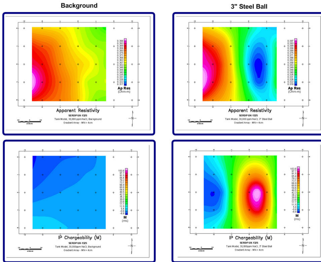
Figure 3.07: Summary plot showing apparent resistivity and IP chargeability for background and 3" steel ball target immersed in a solution of 30,000 ppm NaCl ( \rho=0.236 \Omega\text{-m} ).
