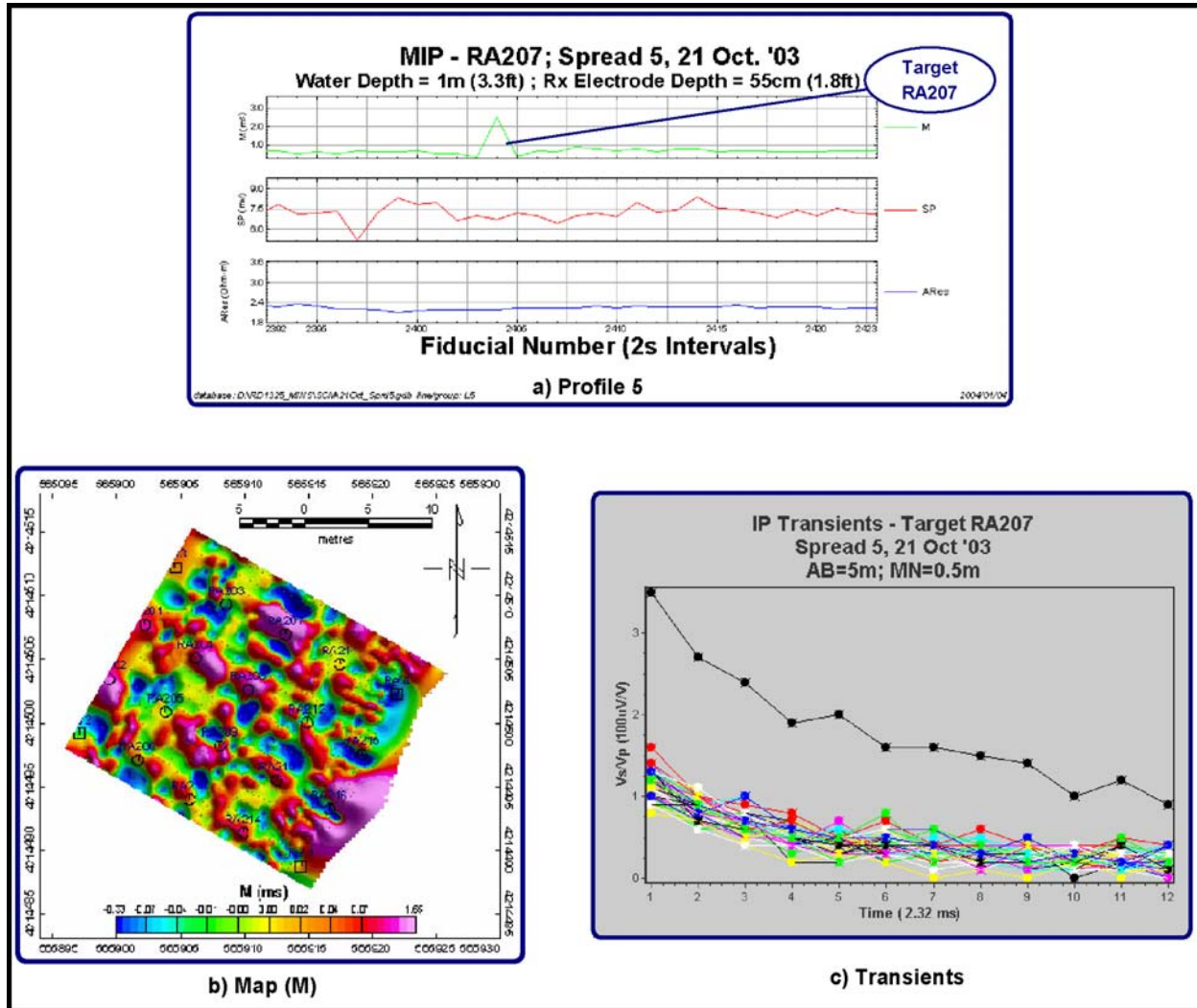
Figure 5.05: Composite figure showing center-line profile over target RA207 (a), color intensity map of leveled chargeability (M), and IP decay transients over target RA207 (c). Data is from Spread 5, water
