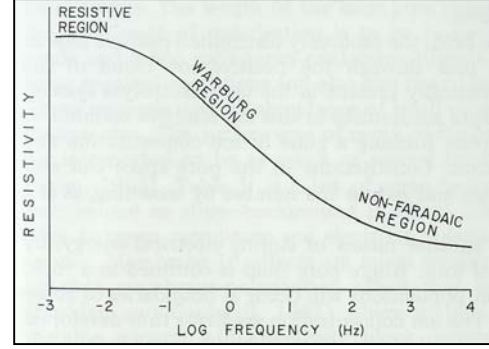
Figure 2.02: Idealized spectrum depicting the frequency behavior of the impedance across an electrode boundary. (Sumner, [4])
