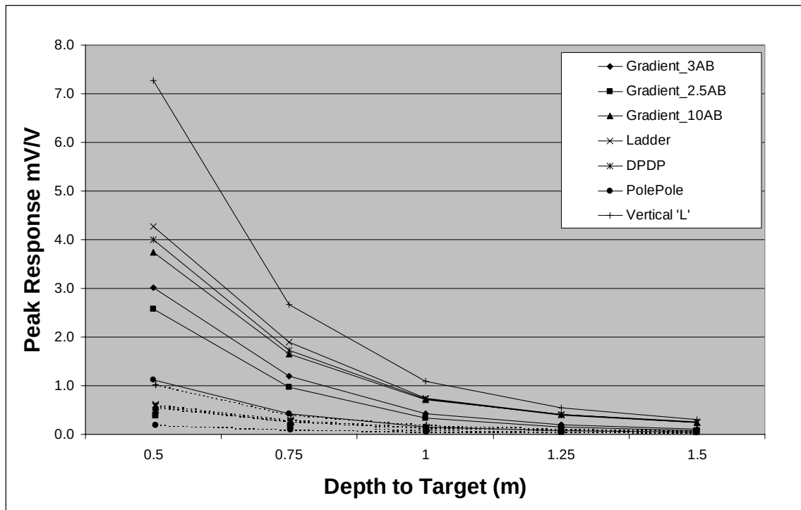
Figure 3.18: Peak IP response as a function of target depth for different electrode arrays. Curves with solid lines represent a salt water host while the dashed curves are results for fresh water.
