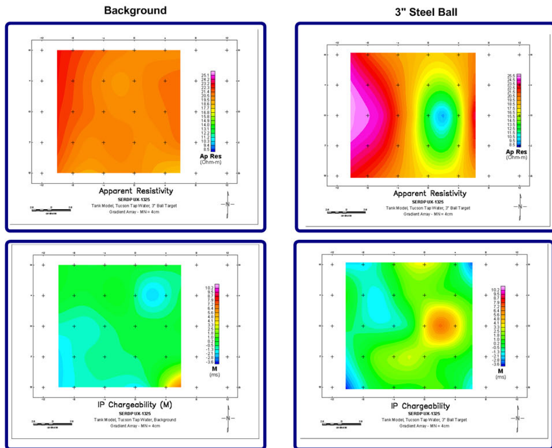
Figure 3.04: Summary plot showing apparent resistivity and IP chargeability for background and 3" steel ball target in Tucson tap water ( \rho=26 \Omega\text{-m} )
