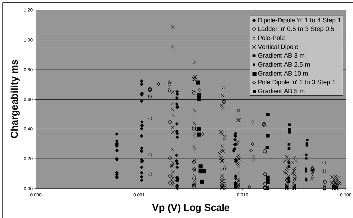
Figure 3.19: Comparison of IP response and primary voltage ( V_p ) for various array geometries.
