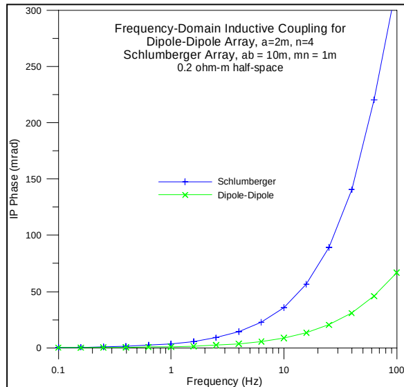
Figure 2.10a: Electromagnetic coupling – Frequency Domain
