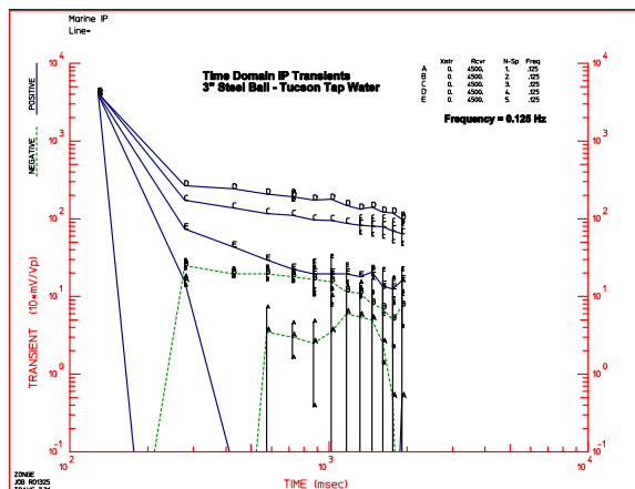
Figure 3.05: IP decay transients measured over the central profile for a 3” steel ball in Tucson tap water.
