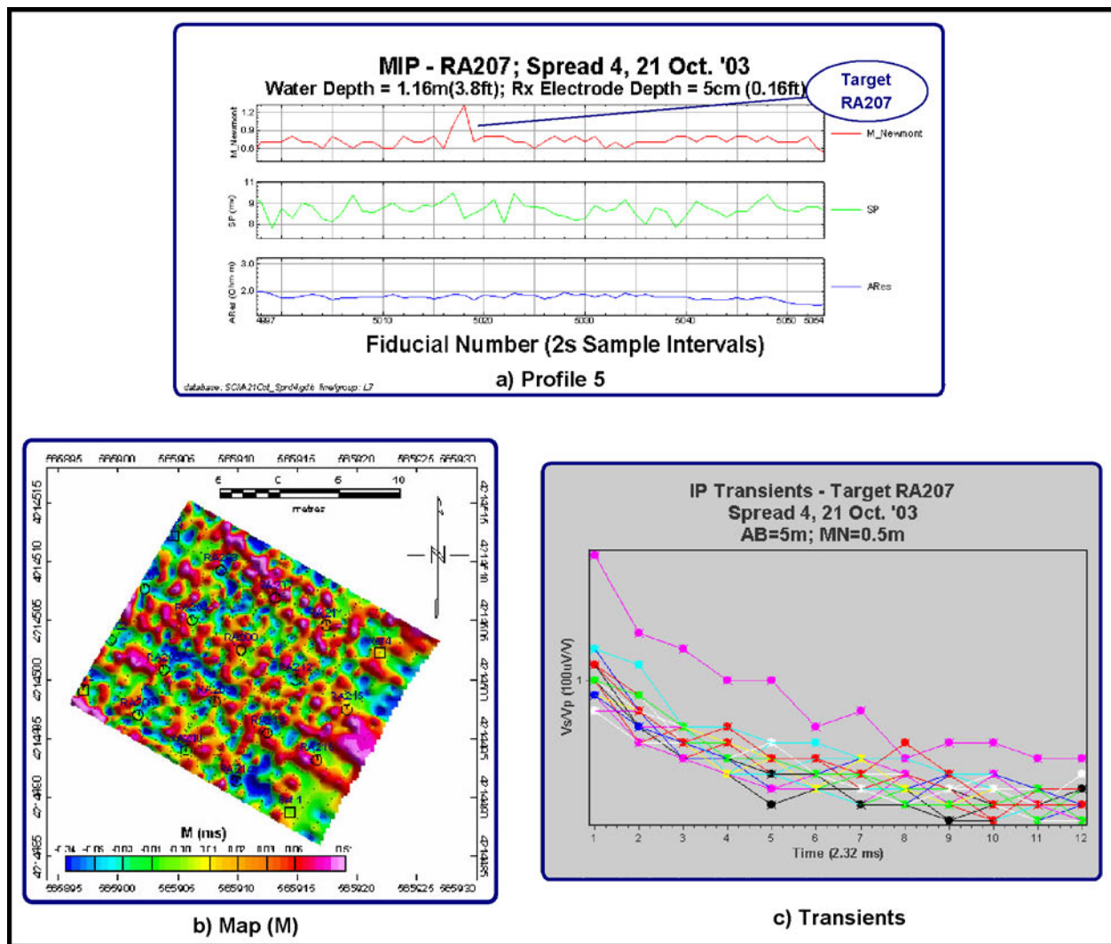
Figure 5.04: Composite figure showing center-line profile over target RA207 (a), color intensity map of leveled chargeability (M), and IP decay transients over target RA207 (c). Data are from Spread 4, water depth 1.16 m, Rx electrode depth 5 cm.
