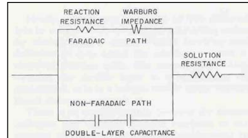
Figure 2.01: Equivalent circuit representing impedance across an electrode boundary. (After Sumner [4])
