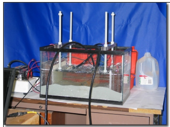
Figure 3.01: Photograph of aquarium used in scale-model experiments.
