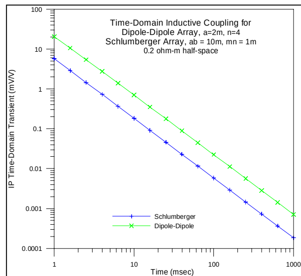
Figure 2.10b: Electromagnetic coupling – Time Domain.
