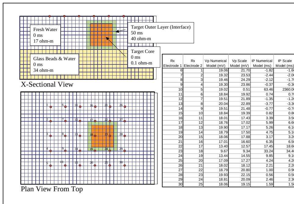
Figure 3.10: Numerical model calibration to 3" steel ball model immersed in Tucson tap water (inhomogeneous target case).
