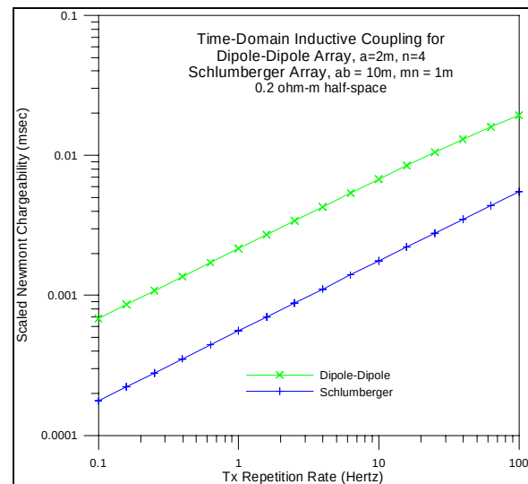
Figure 2.11: Time domain EM coupling as measured by the scaled chargeability parameter ( M_1 ) as a function of repetition rate (i.e., 1/T )
