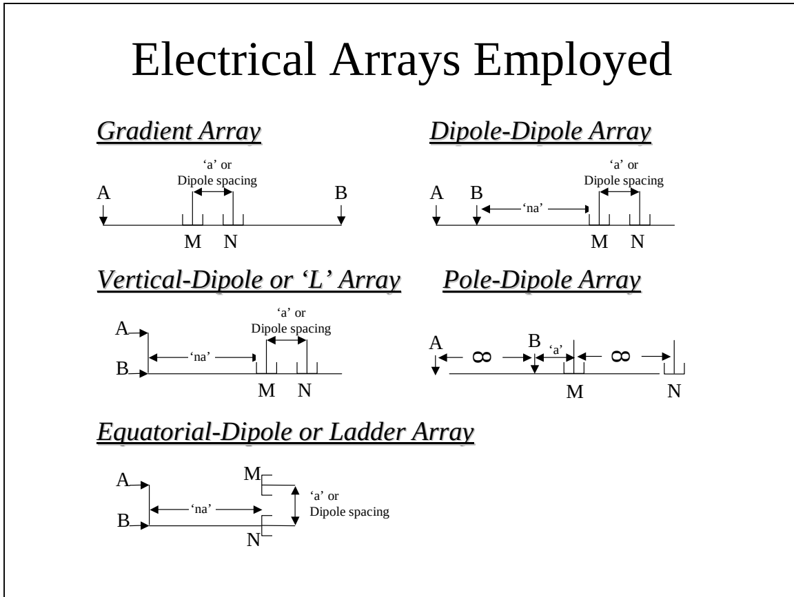
Figure 3.17: Array geometries employed during numerical model study.
