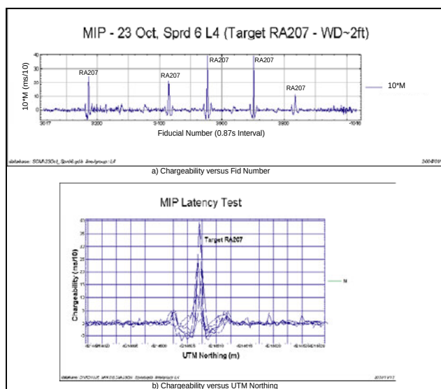
Figure 5.11: Latency check – Multiple passes over target RA207.
