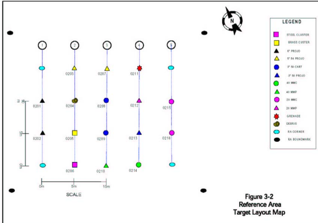
Figure 5.02: Reference area target map. (Figure 3-2 in [20])
