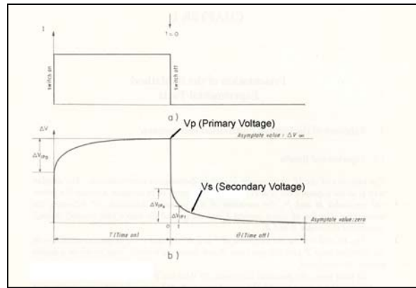
Figure 2.06: Schematic depiction of the IP phenomenon as seen in the time domain. (adapted from Bertin and Loeb [2])
