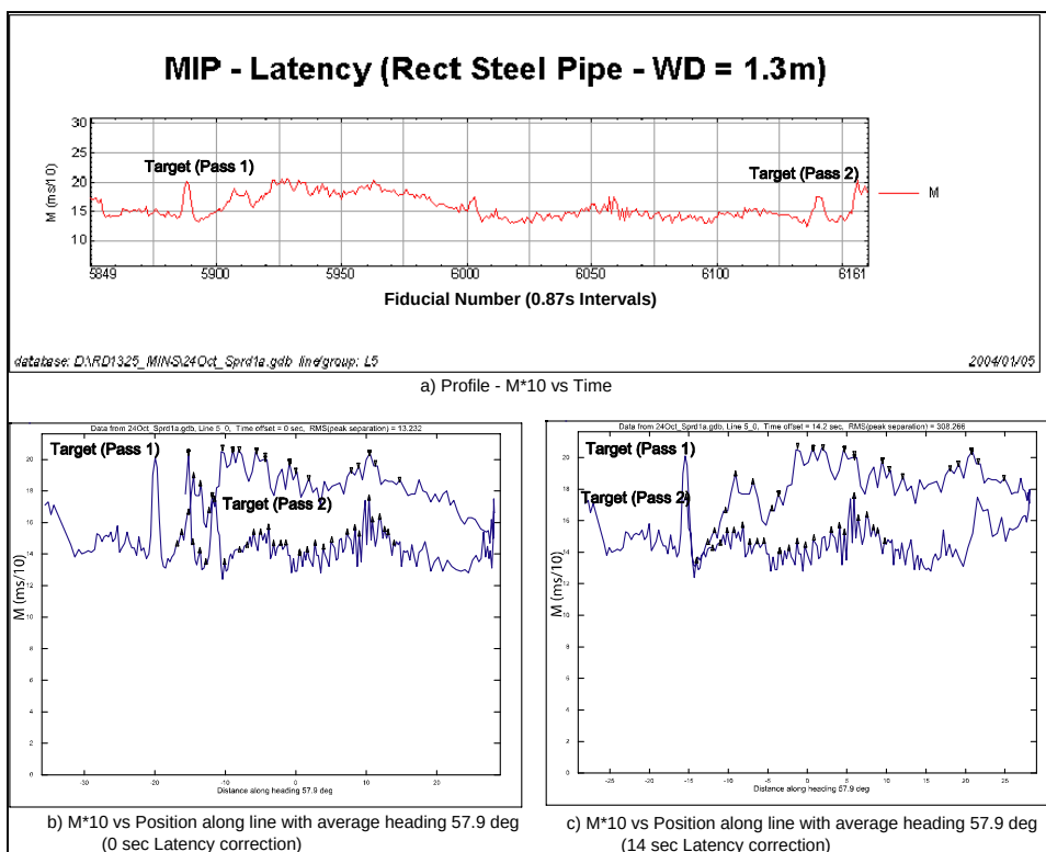
Figure 5.10: Summary diagram of latency test using 2-ft length of steel (shown in Fig. 5.09). The results show a timing correction of 14s is required.
