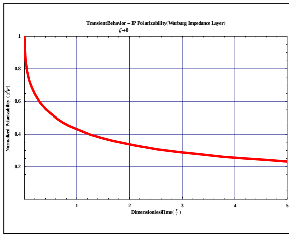
Figure 2.05: Parametric plot showing relative time-domain IP polarizability as a function of time with \xi=0 . The results are based on a Warburg model of Faradaic electrode impedance
