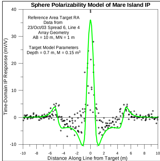
Figure 5.12: Isotropic dipole model fit to the profile data shown in Figure 5.11 for target RA207.
