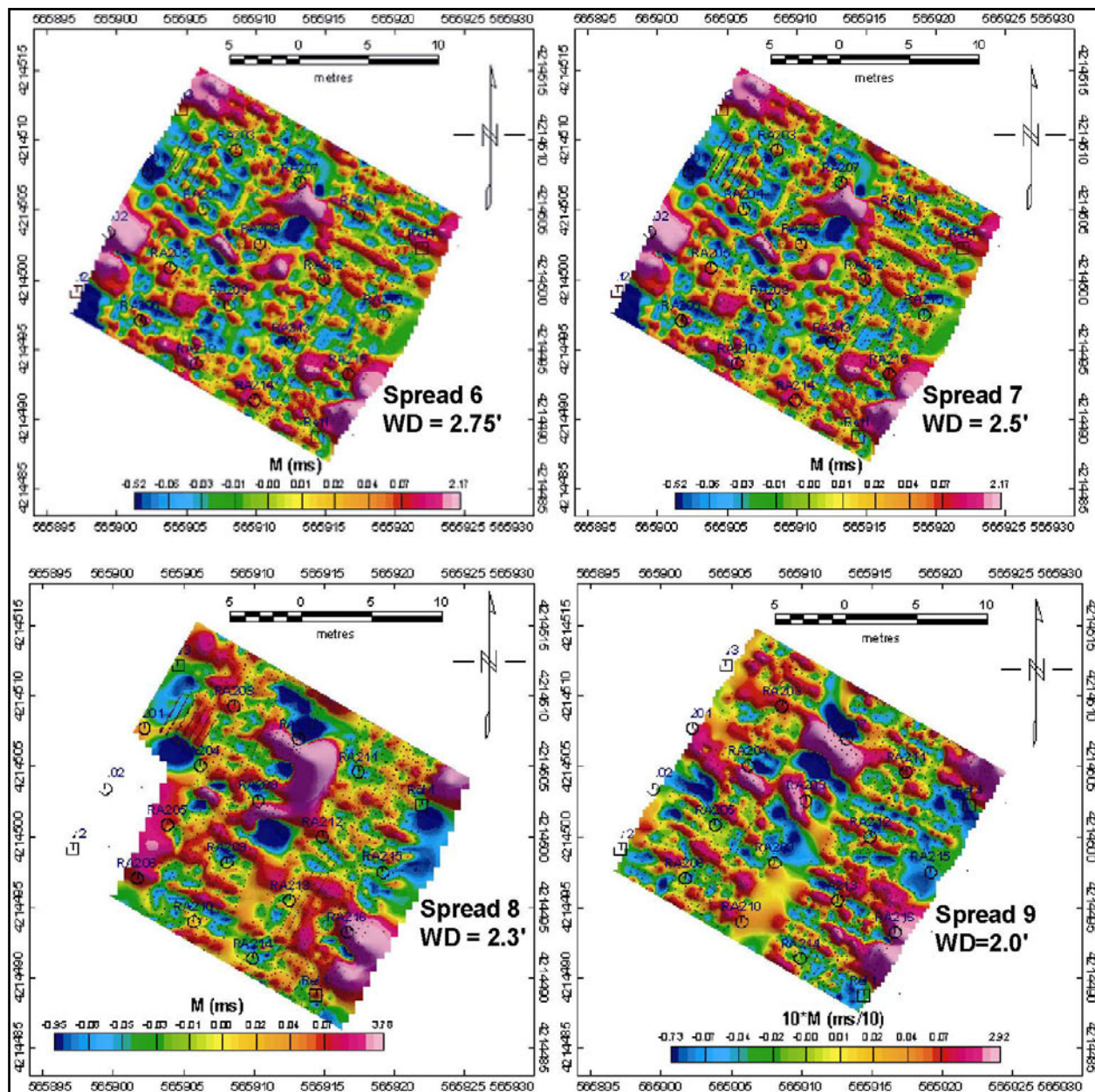
Figure 5.07: Sequence of 4 spreads illustrating progressive improvement in SNR as the water level decreases. AB = 5m, MN = 0.5m, Rx electrode depth = 55cm; sample interval 1s.
