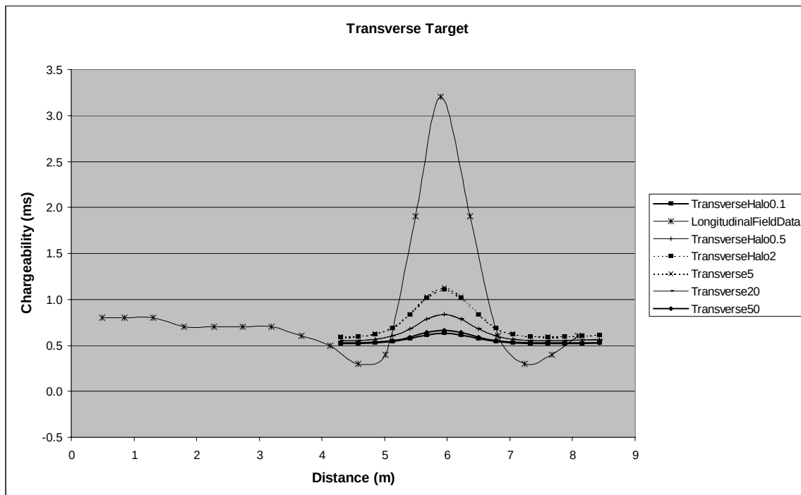
Figure 3.14: Comparative transverse responses for the model shown in Figure 3.13.
