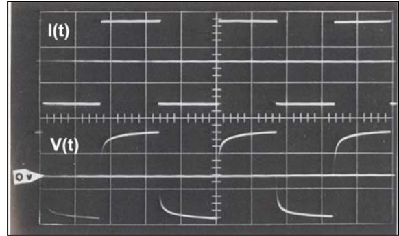
Figure 2.09: Typical current and voltage waveforms for a frequency domain IP measurement.
