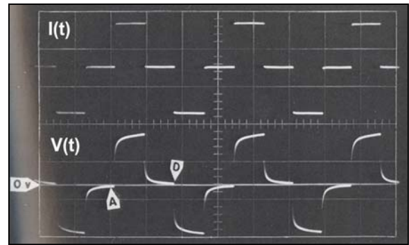
Figure 2.07: Oscillographs showing current waveform (top) and voltage waveform (bottom) for time domain IP. (after Sumner, [3])
