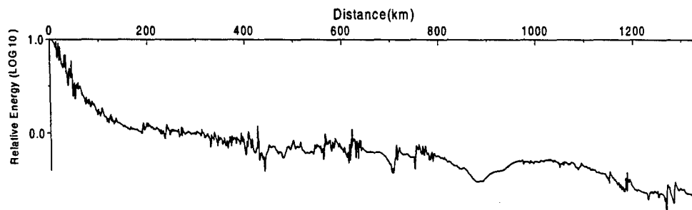
Energy attenuation versus distance
