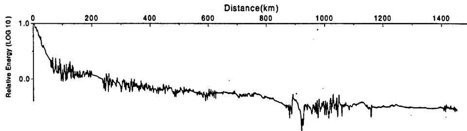
Energy attenuation versus distance
