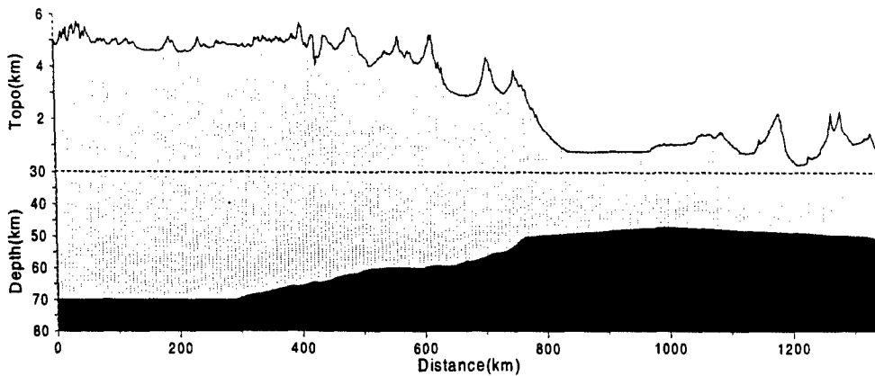
A sample profile from epicenter to WMQ of the June 2, 1990 event.
