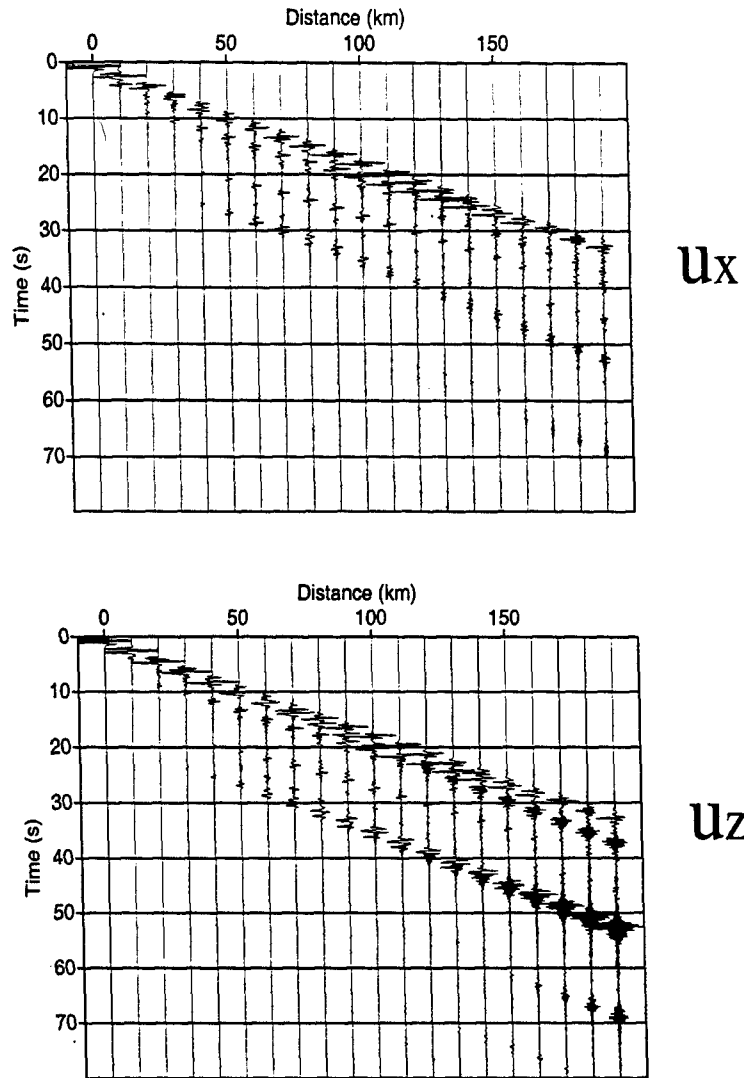
Figure 17. Synthetic seismograms for Flora-Asnes crust model (Table 1). An explosive source is located at a depth of 2\text{km} and the source time function has a dominant frequency of 2\text{Hz}
