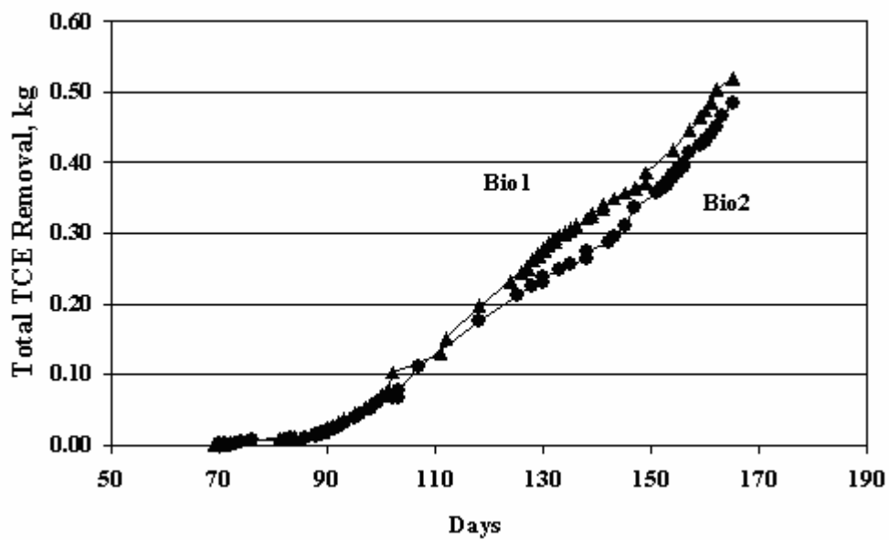
Fig. 8 Mass of TCE removed by biological treatment.
