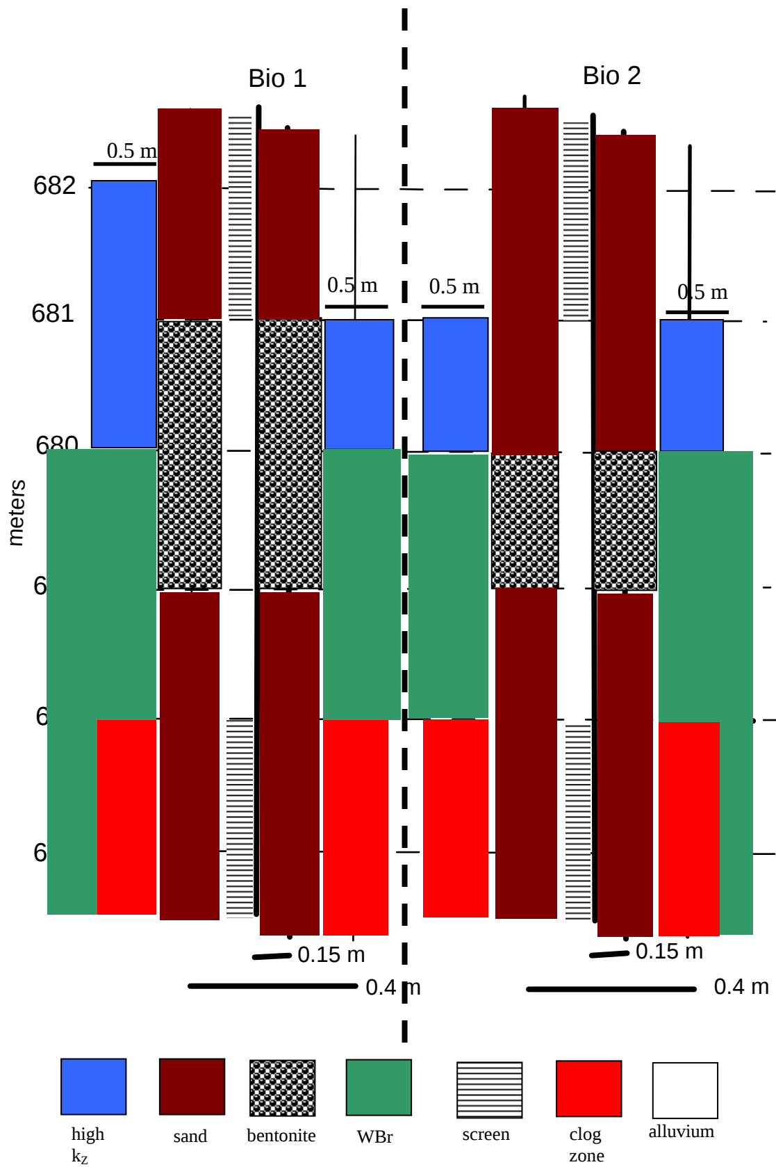
Fig. 20 Model conceptualization of well pack at biotreatment wells one and two. The “clogging” zones extend for 0.5 meters around the gravel pack of the lower wellscreens.
