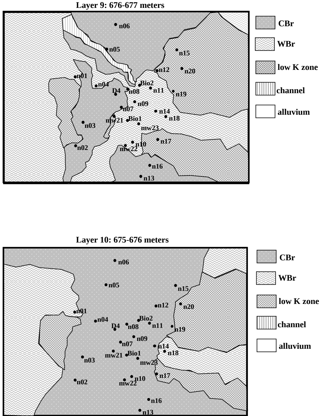
Fig. 14 Model material types for layers 9 and 10. CBr is the competent bedrock and WBr is the weathered bedrock. The channel represents a highly fractured zone between bioremediation well two and monitoring location N05.
