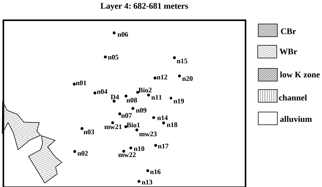
Fig. 11 Model material types for layers 1 through 4. CBr is the competent bedrock and WBr is the weathered bedrock. The channel represents a highly fractured zone between bioremediation well two and monitoring location N05.
