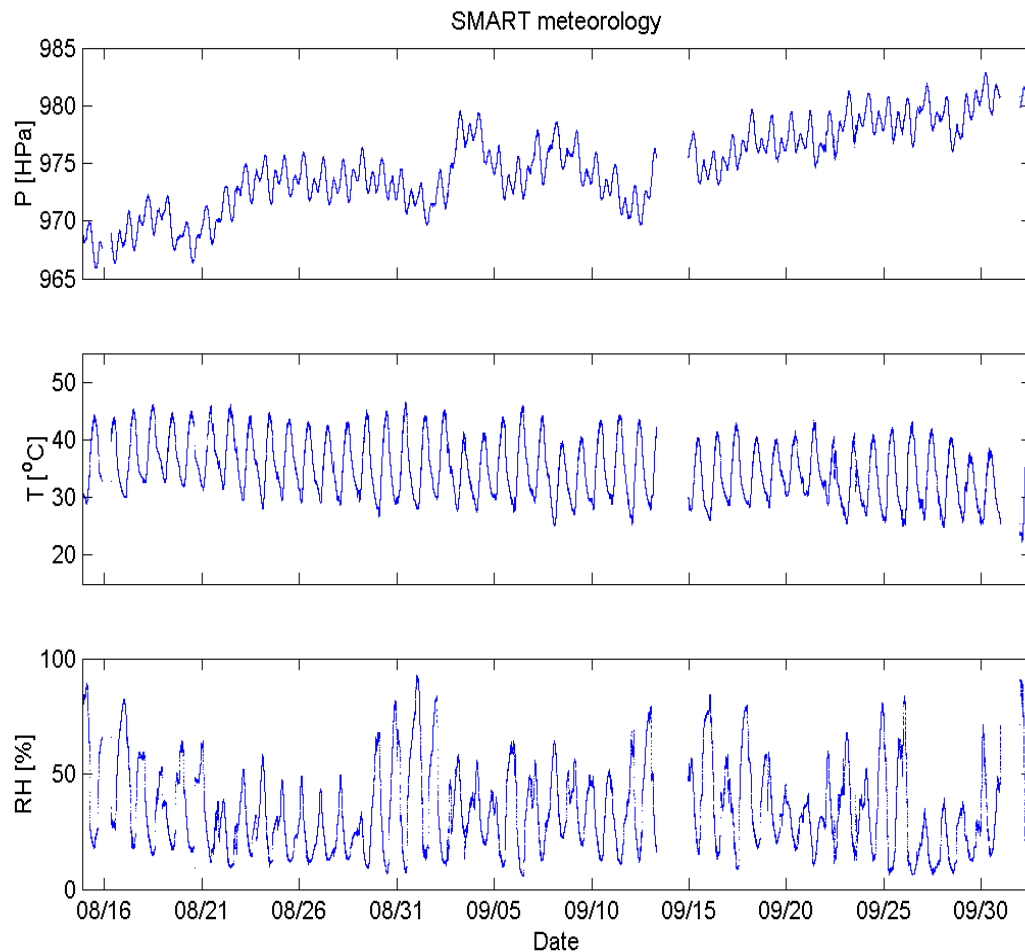
Figure J.5 Air pressure, temperature, and relative humidity measured near the ground surface
