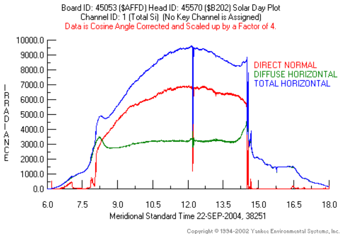
Figure J.4 An output from the shadowband radiometer.
