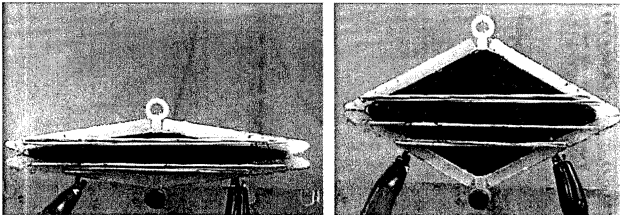
Figure 10: Experimental dielectric elastomer actuator showing 200 percent strain.
