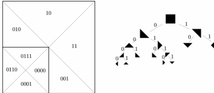
Figure 5: The binary tree representation of a RTIN partition.
