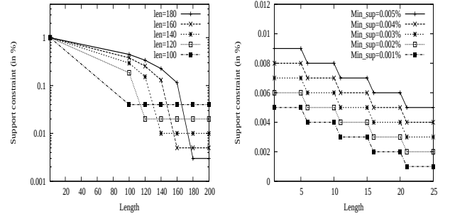
Fig. 8. Support constraint ( gazelle ). Fig. 9. Support constraint ( T10I4D100K ).
