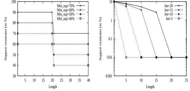
Fig. 6. Support constraint ( pumsb ). Fig. 7. Support constraint ( mushroom ).
