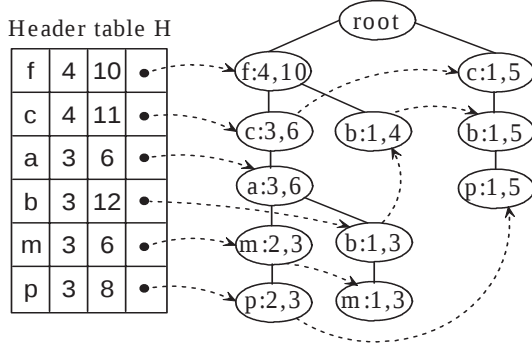
Figure 1: The FP-tree of our running example.
