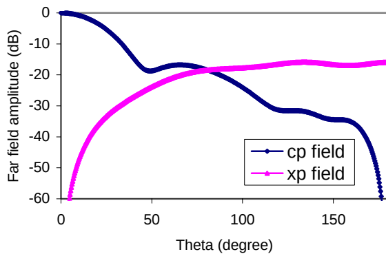
Fig 6: Co-polarized (cp) and cross-polarized (xp) field obtained for the elliptical aperture with \phi = 45^\circ and excited with TE_{11} mode, before the improvement of the conditioning.
